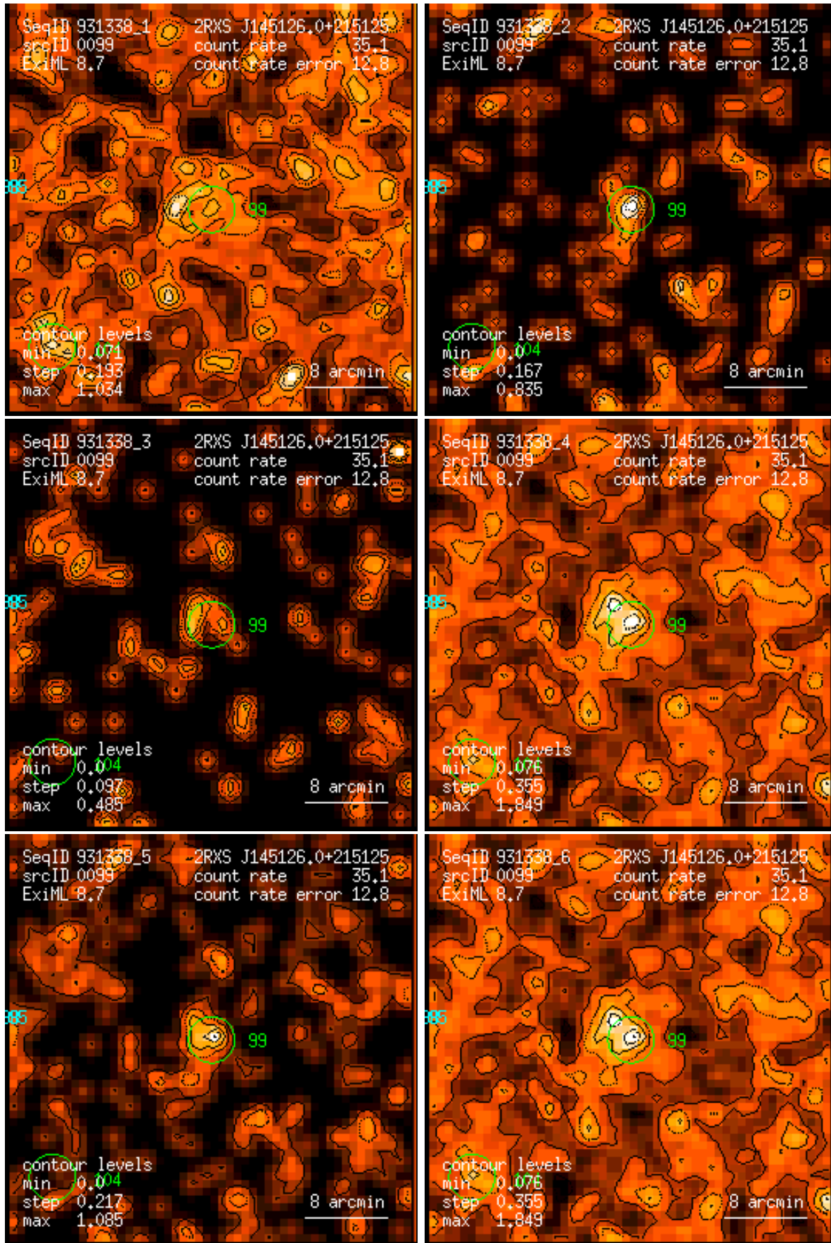
Figure 99: RASS 931338: detection 0099: band rate images, Gaussian filter: (1) PSPC channels 11 – 41, (2) 52 – 90, (3) 91 – 201, (4) 11 – 235, (5) 52 – 201, (6) 11 – 201. Broad band rates in counts/ks. Band rate contour levels in counts/ks/arcmin 2 .
