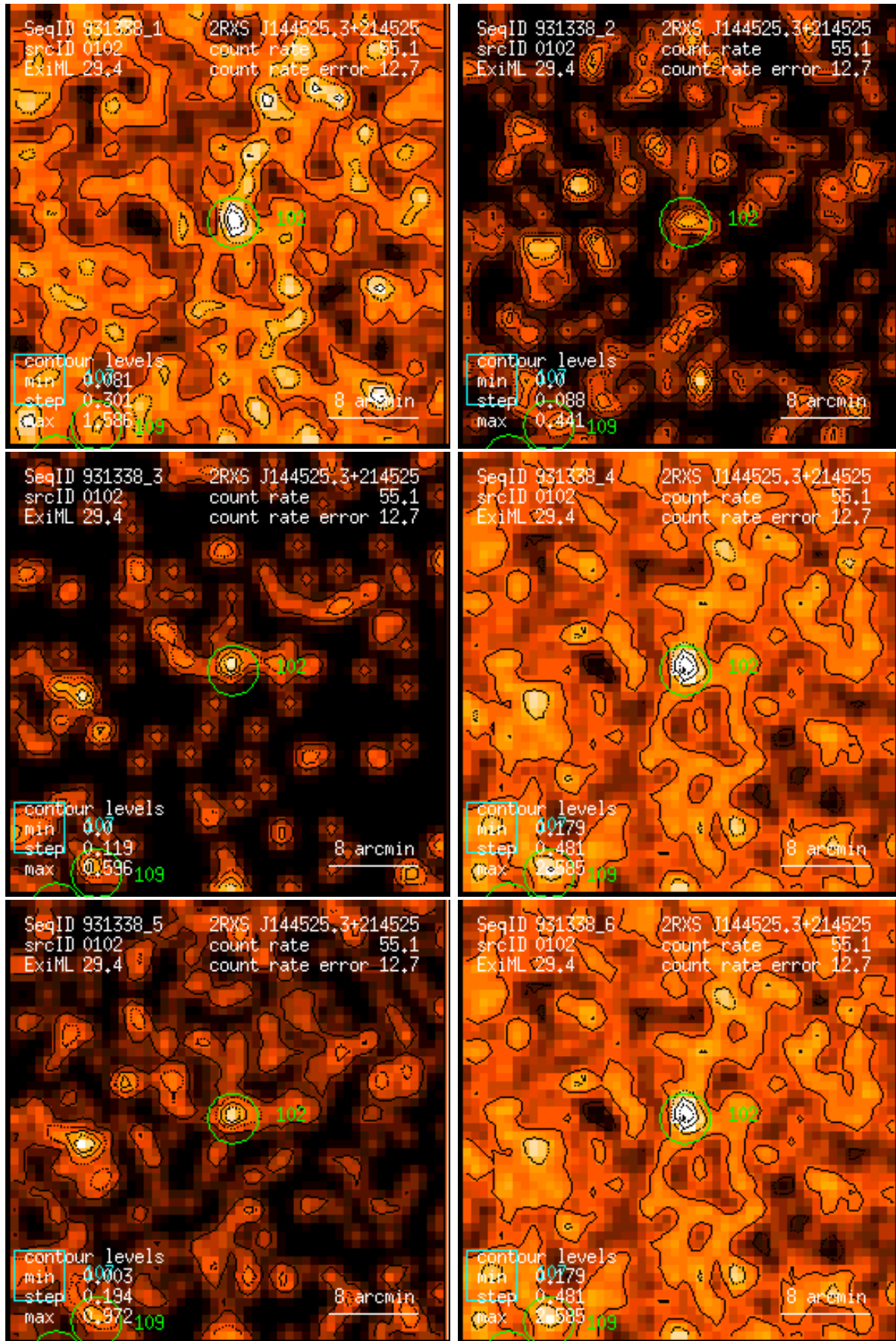
Figure 102: RASS 931338: detection 0102: band rate images, Gaussian filter: (1) PSPC channels 11 – 41, (2) 52 – 90, (3) 91 – 201, (4) 11 – 235, (5) 52 – 201, (6) 11 – 201. Broad band rates in counts/ks. Band rate contour levels in counts/ks/arcmin 2 .
