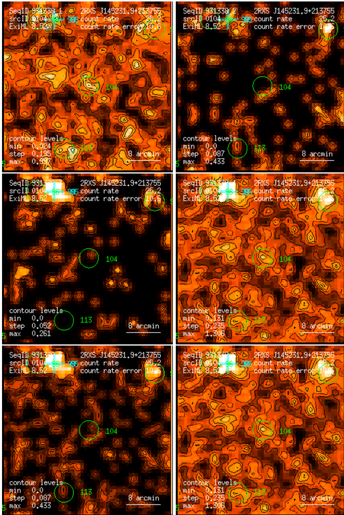
Figure 104: RASS 931338: detection 0104: band rate images, Gaussian filter: (1) PSPC channels 11 – 41, (2) 52 – 90, (3) 91 – 201, (4) 11 – 235, (5) 52 – 201, (6) 11 – 201. Broad band rates in counts/ks. Band rate contour levels in counts/ks/arcmin 2 .
