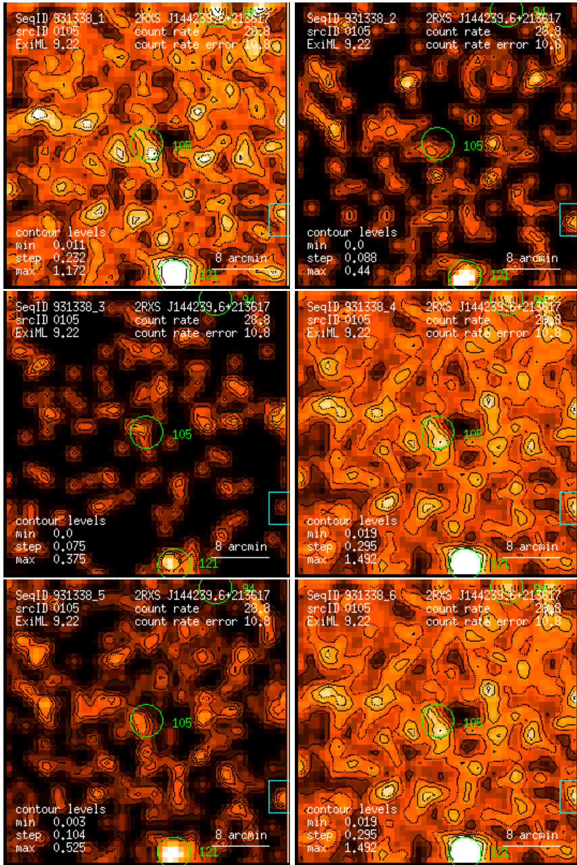
Figure 105: RASS 931338: detection 0105: band rate images, Gaussian filter: (1) PSPC channels 11 – 41, (2) 52 – 90, (3) 91 – 201, (4) 11 – 235, (5) 52 – 201, (6) 11 – 201. Broad band rates in counts/ks. Band rate contour levels in counts/ks/arcmin 2 .
