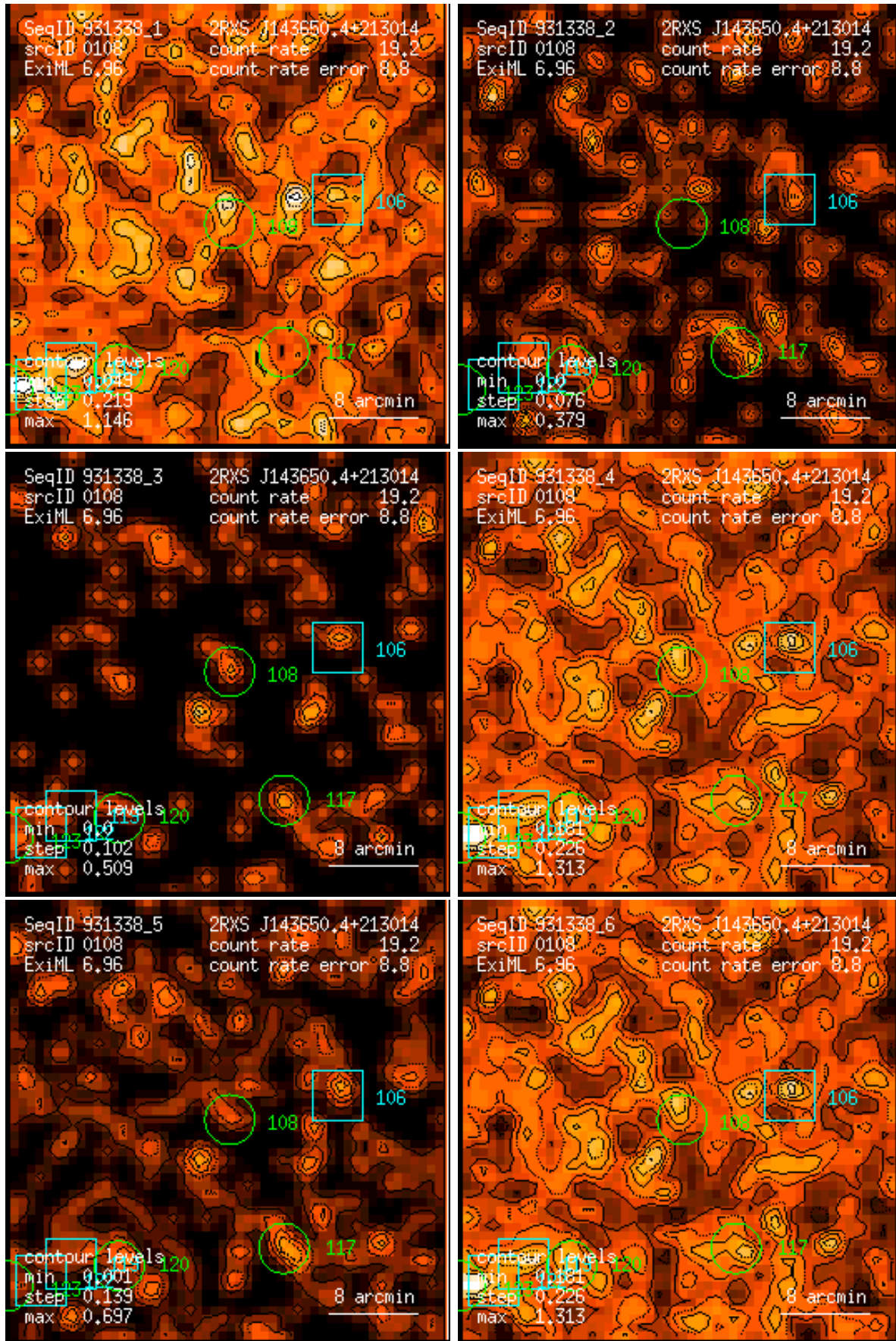
Figure 108: RASS 931338: detection 0108: band rate images, Gaussian filter: (1) PSPC channels 11 – 41, (2) 52 – 90, (3) 91 – 201, (4) 11 – 235, (5) 52 – 201, (6) 11 – 201. Broad band rates in counts/ks. Band rate contour levels in counts/ks/arcmin 2 .
