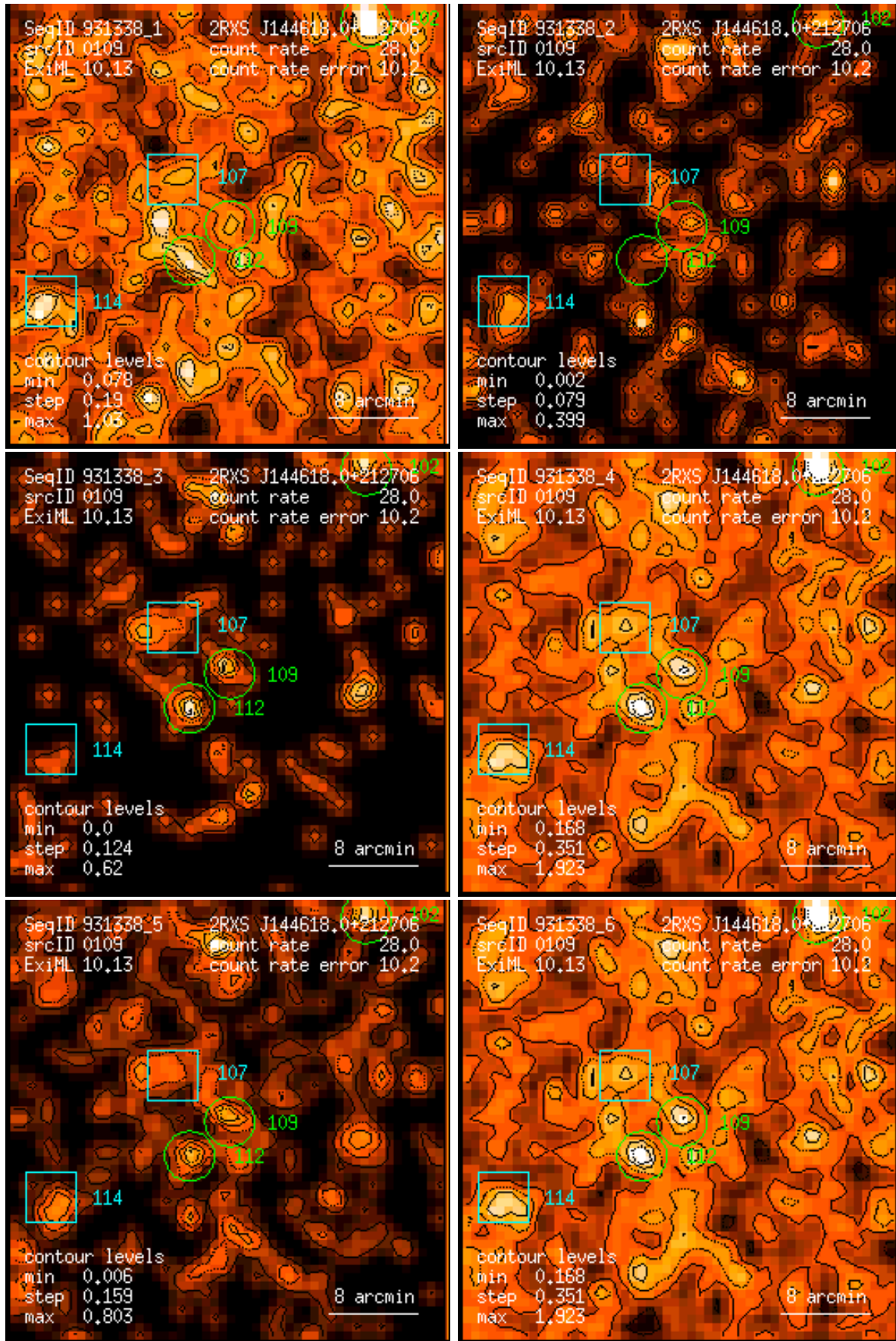
Figure 109: RASS 931338: detection 0109: band rate images, Gaussian filter: (1) PSPC channels 11 – 41, (2) 52 – 90, (3) 91 – 201, (4) 11 – 235, (5) 52 – 201, (6) 11 – 201. Broad band rates in counts/ks. Band rate contour levels in counts/ks/arcmin 2 .
