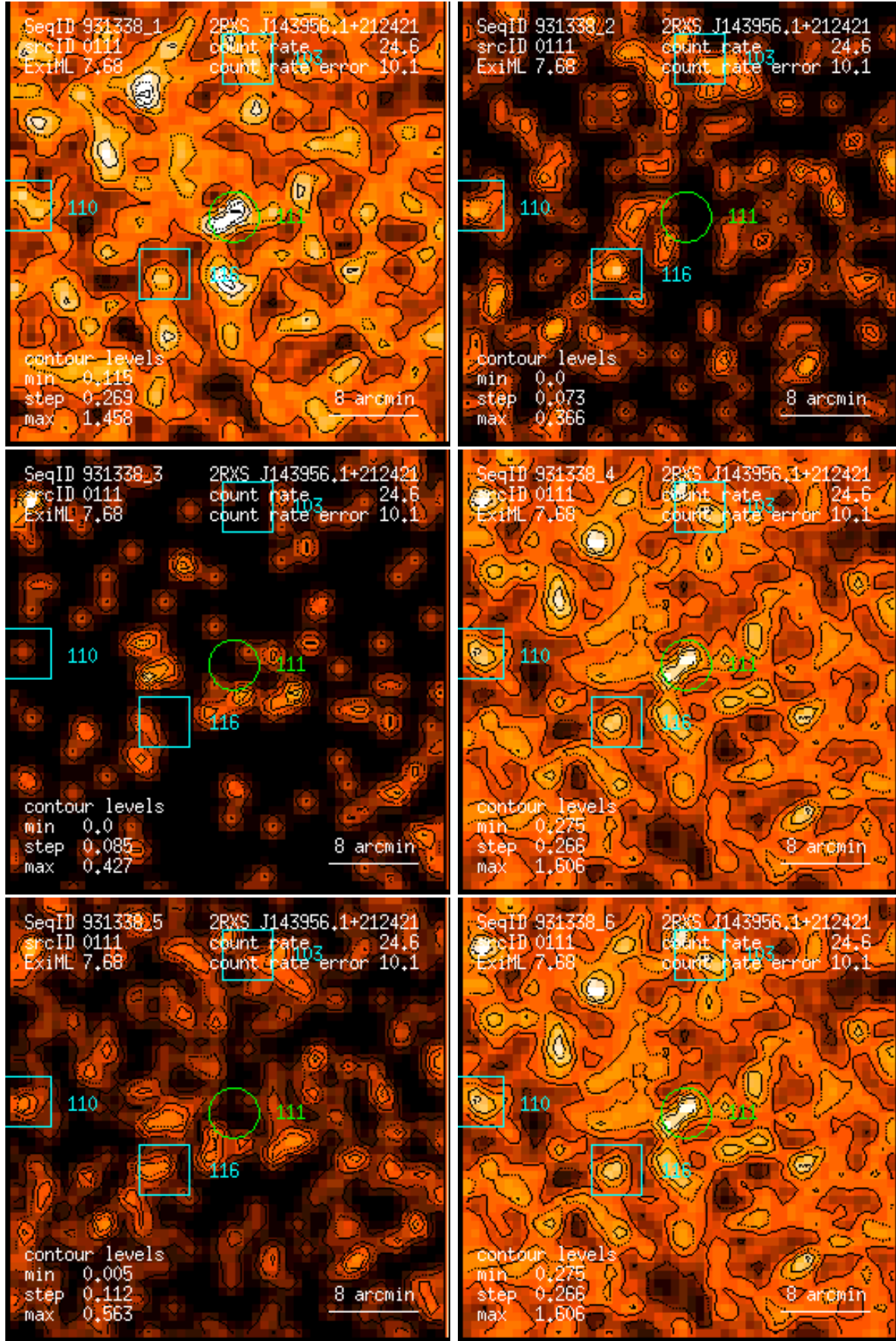
Figure 111: RASS 931338: detection 0111: band rate images, Gaussian filter: (1) PSPC channels 11 – 41, (2) 52 – 90, (3) 91 – 201, (4) 11 – 235, (5) 52 – 201, (6) 11 – 201. Broad band rates in counts/ks. Band rate contour levels in counts/ks/arcmin 2 .
