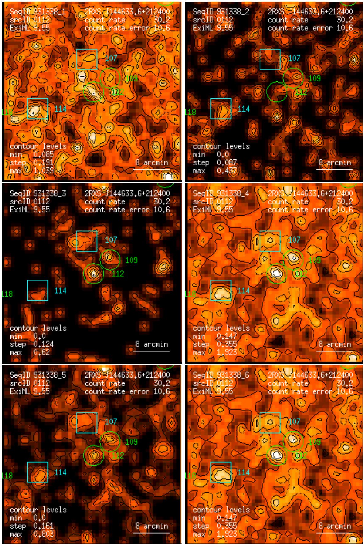
Figure 112: RASS 931338: detection 0112: band rate images, Gaussian filter: (1) PSPC channels 11 – 41, (2) 52 – 90, (3) 91 – 201, (4) 11 – 235, (5) 52 – 201, (6) 11 – 201. Broad band rates in counts/ks. Band rate contour levels in counts/ks/arcmin 2 .
