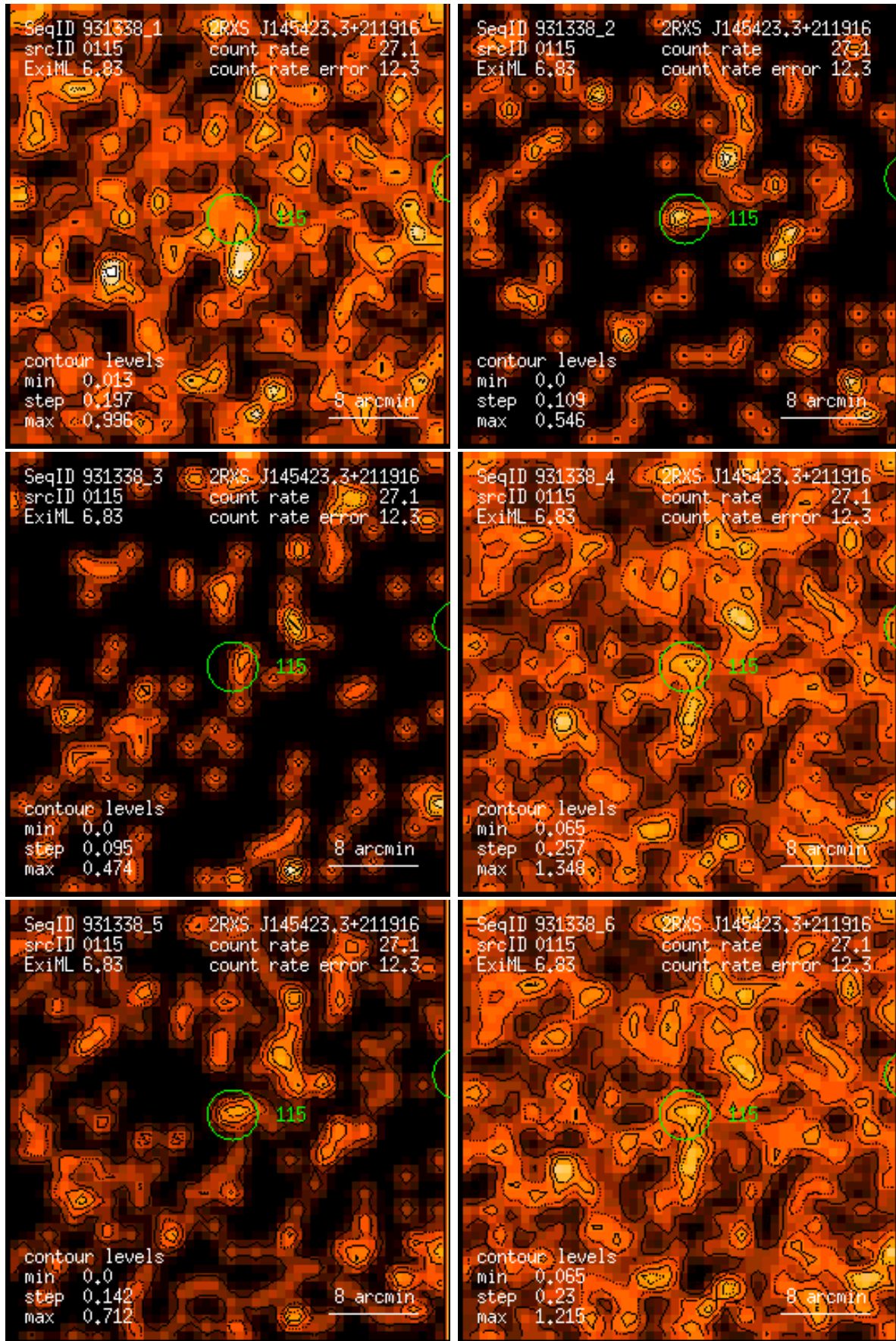
Figure 115: RASS 931338: detection 0115: band rate images, Gaussian filter: (1) PSPC channels 11 – 41, (2) 52 – 90, (3) 91 – 201, (4) 11 – 235, (5) 52 – 201, (6) 11 – 201. Broad band rates in counts/ks. Band rate contour levels in counts/ks/arcmin 2 .
