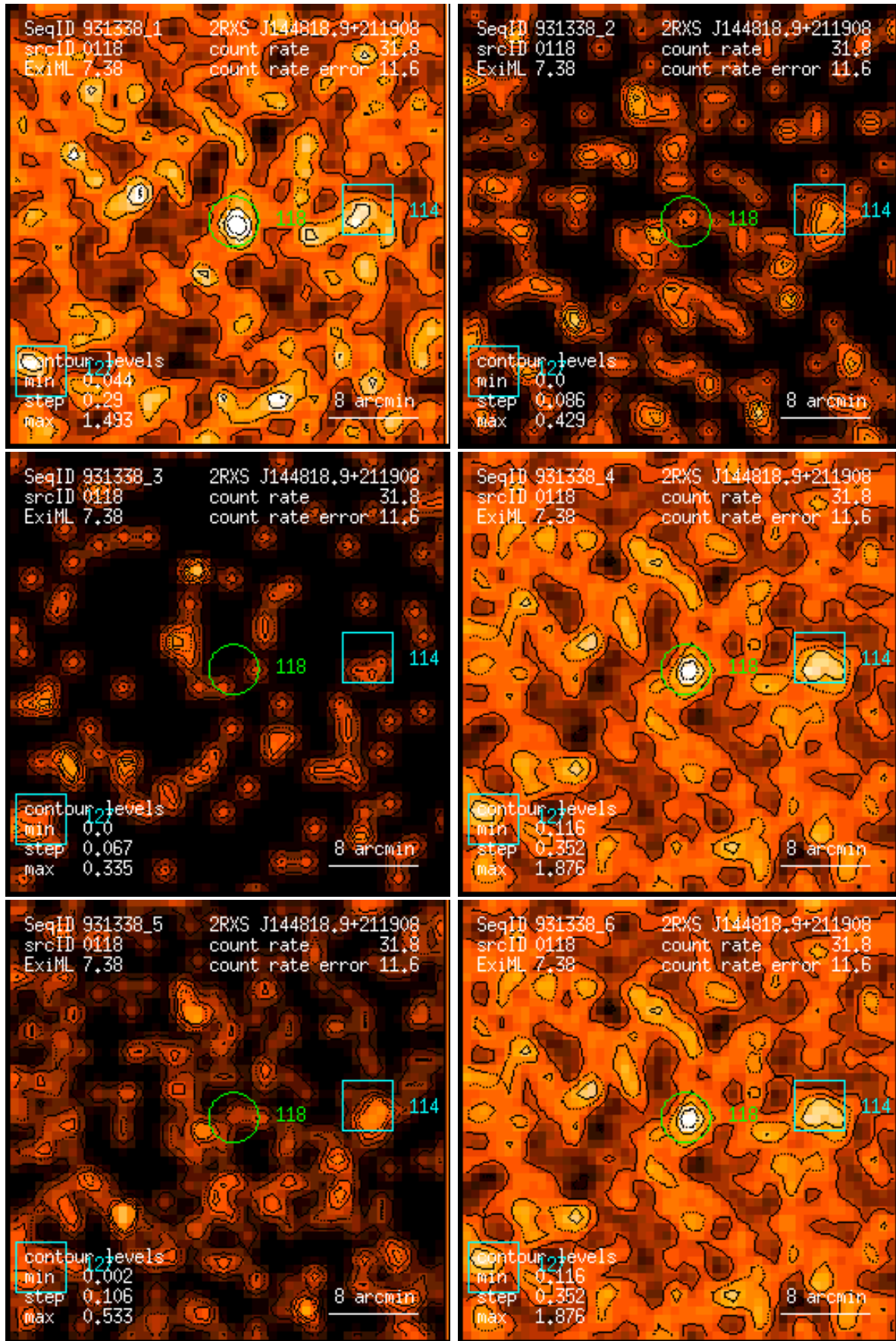
Figure 118: RASS 931338: detection 0118: band rate images, Gaussian filter: (1) PSPC channels 11 – 41, (2) 52 – 90, (3) 91 – 201, (4) 11 – 235, (5) 52 – 201, (6) 11 – 201. Broad band rates in counts/ks. Band rate contour levels in counts/ks/arcmin 2 .
