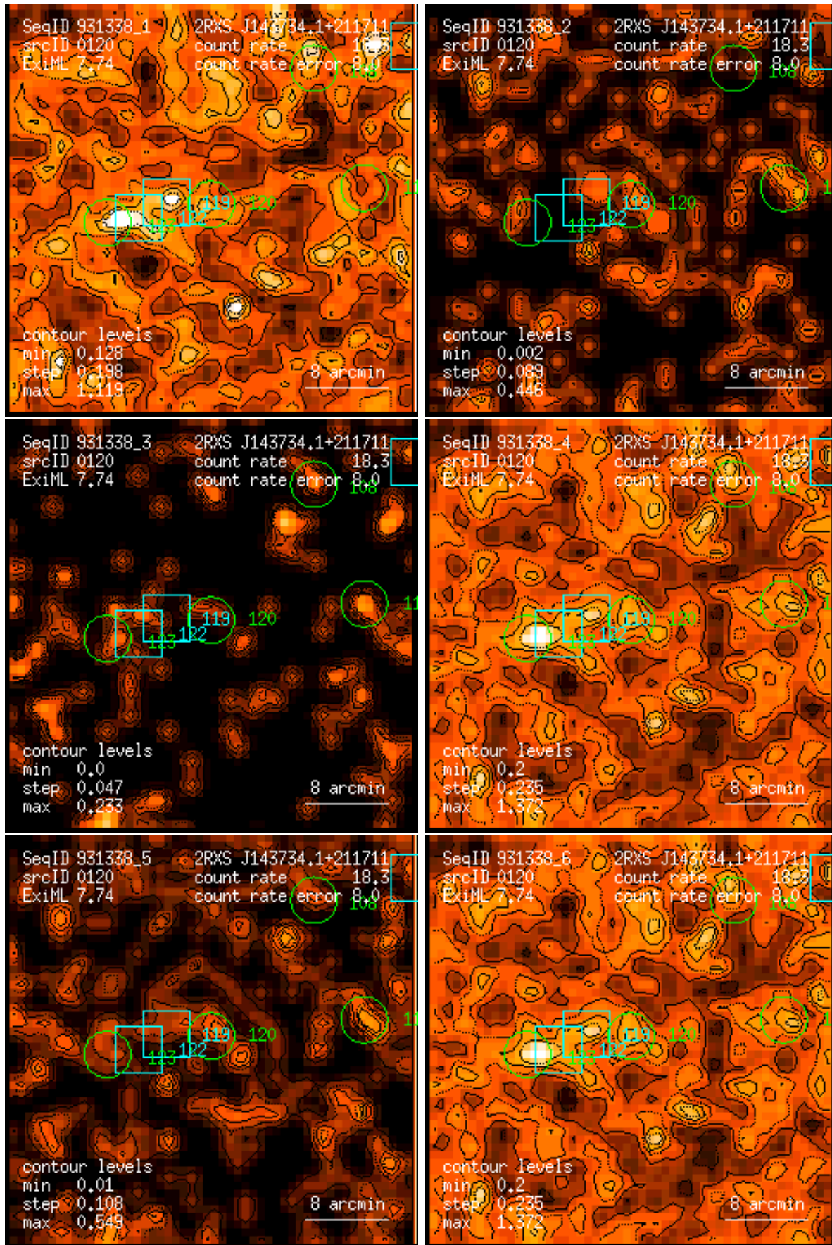
Figure 120: RASS 931338: detection 0120: band rate images, Gaussian filter: (1) PSPC channels 11 – 41, (2) 52 – 90, (3) 91 – 201, (4) 11 – 235, (5) 52 – 201, (6) 11 – 201. Broad band rates in counts/ks. Band rate contour levels in counts/ks/arcmin 2 .
