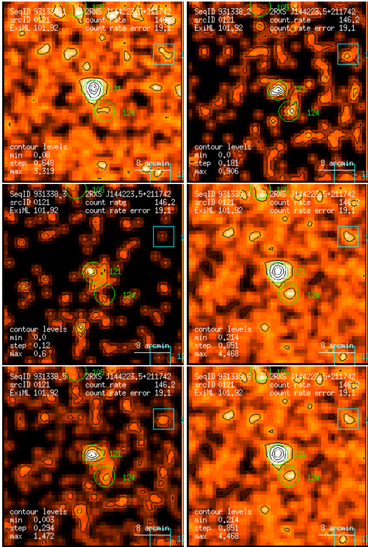
Figure 121: RASS 931338: detection 0121: band rate images, Gaussian filter: (1) PSPC channels 11 – 41, (2) 52 – 90, (3) 91 – 201, (4) 11 – 235, (5) 52 – 201, (6) 11 – 201. Broad band rates in counts/ks. Band rate contour levels in counts/ks/arcmin 2 .
