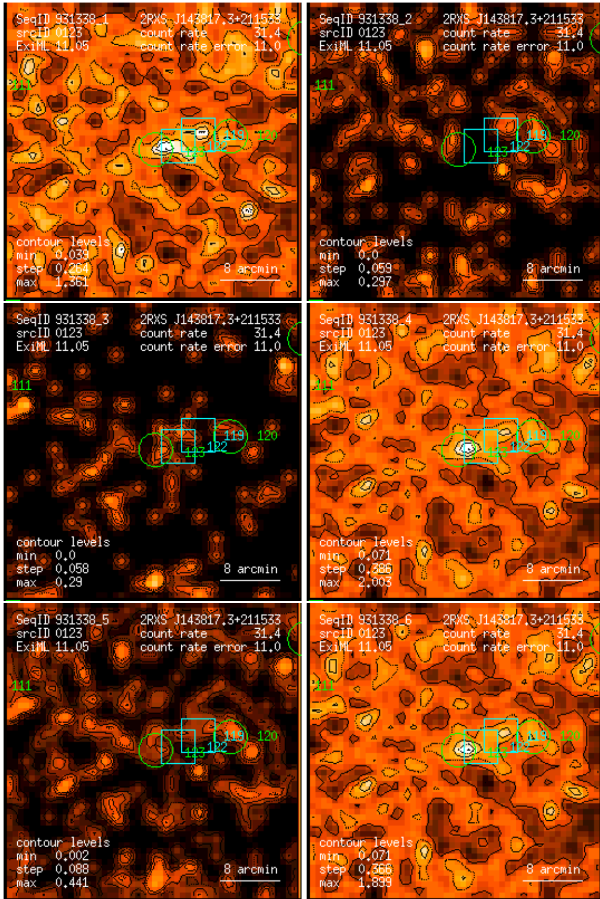
Figure 123: RASS 931338: detection 0123: band rate images, Gaussian filter: (1) PSPC channels 11 – 41, (2) 52 – 90, (3) 91 – 201, (4) 11 – 235, (5) 52 – 201, (6) 11 – 201. Broad band rates in counts/ks. Band rate contour levels in counts/ks/arcmin 2 .
