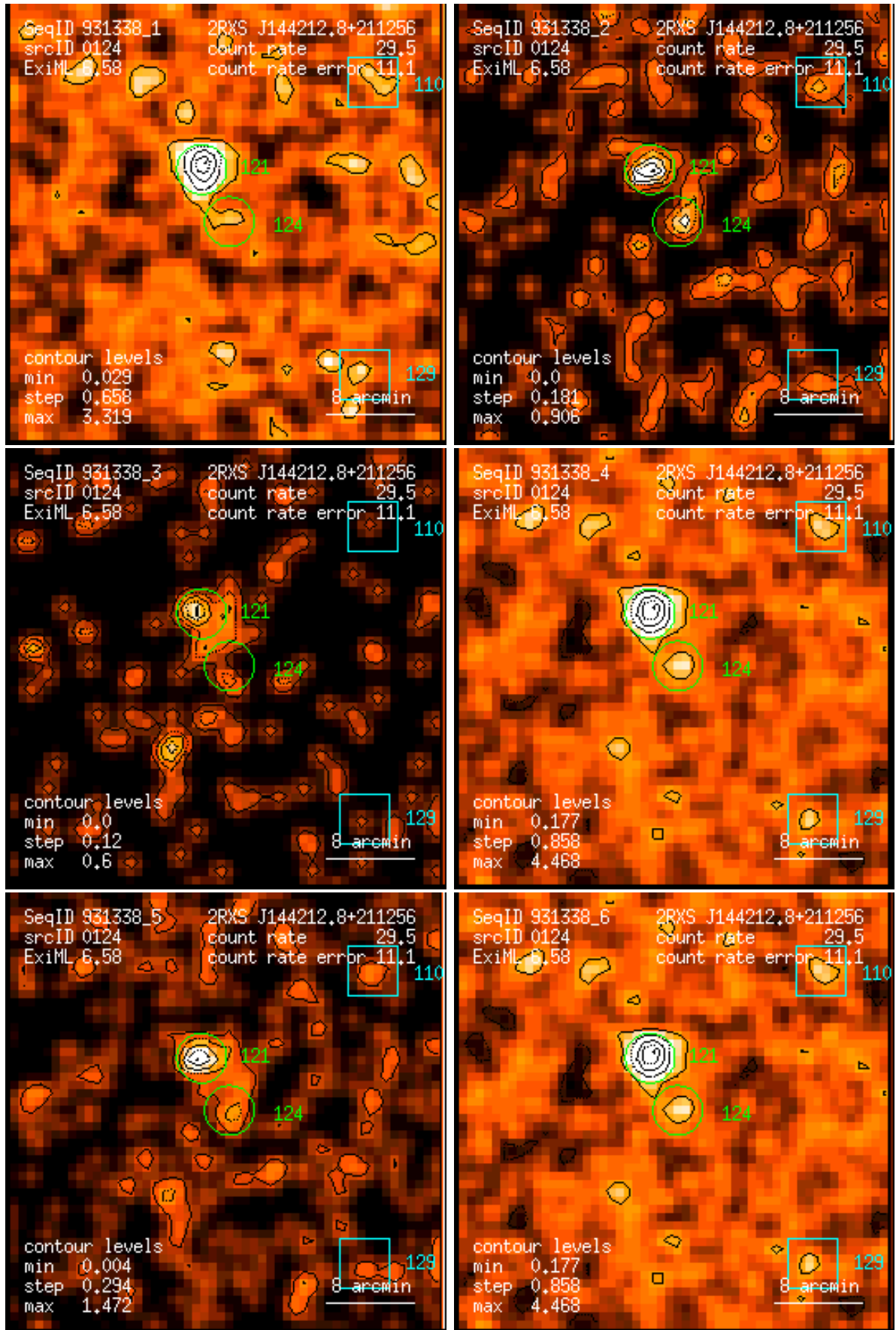
Figure 124: RASS 931338: detection 0124: band rate images, Gaussian filter: (1) PSPC channels 11 – 41, (2) 52 – 90, (3) 91 – 201, (4) 11 – 235, (5) 52 – 201, (6) 11 – 201. Broad band rates in counts/ks. Band rate contour levels in counts/ks/arcmin 2 .
