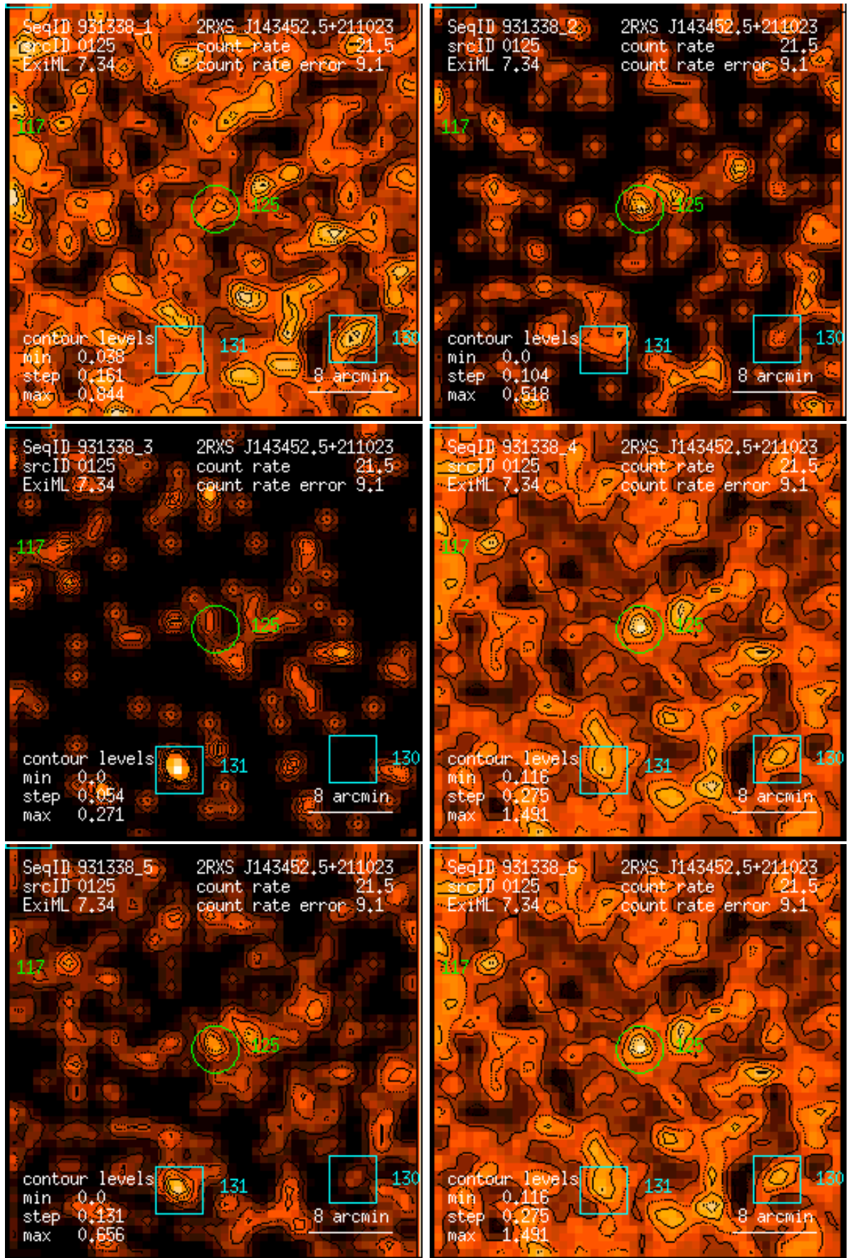
Figure 125: RASS 931338: detection 0125: band rate images, Gaussian filter: (1) PSPC channels 11 – 41, (2) 52 – 90, (3) 91 – 201, (4) 11 – 235, (5) 52 – 201, (6) 11 – 201. Broad band rates in counts/ks. Band rate contour levels in counts/ks/arcmin 2 .
