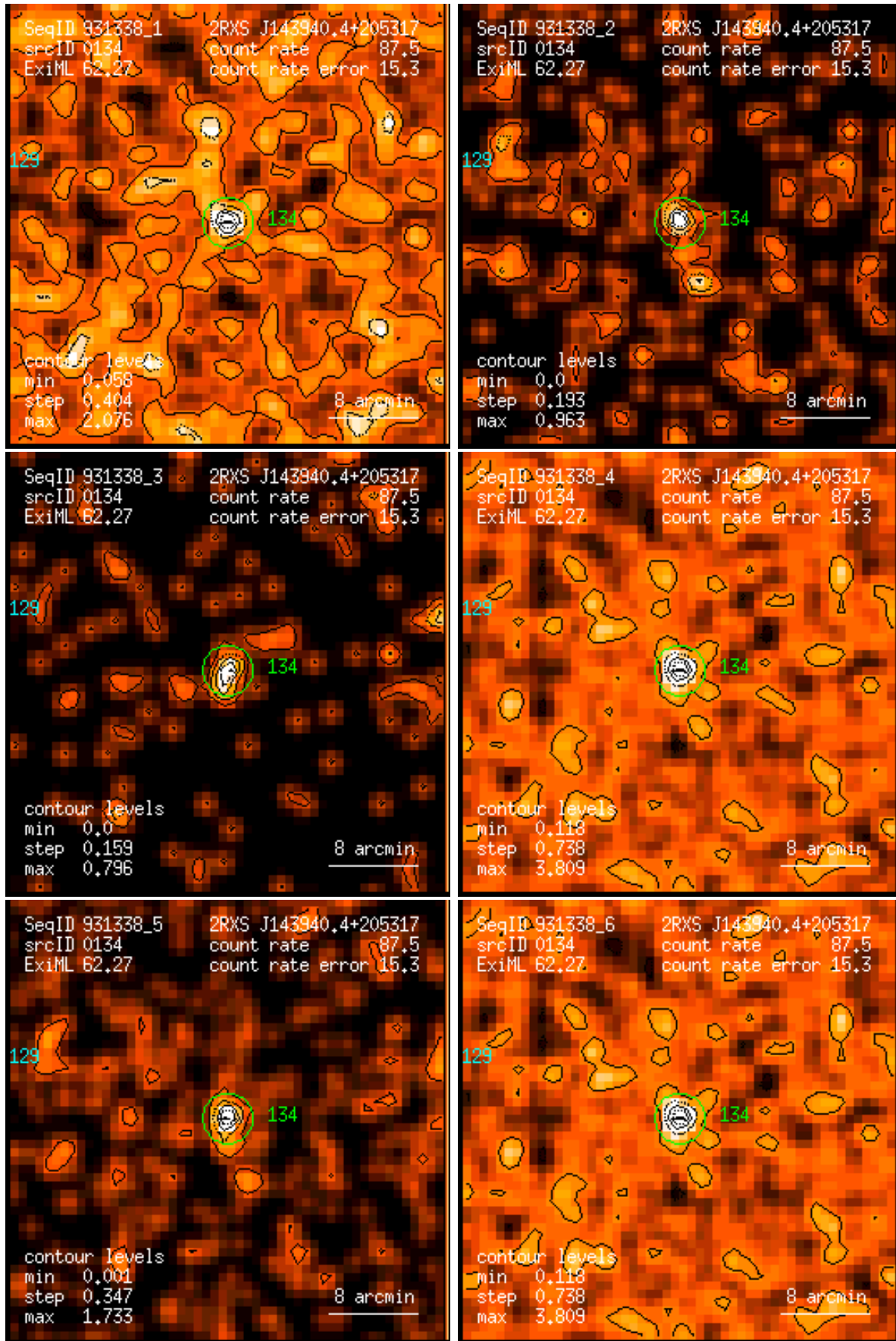
Figure 134: RASS 931338: detection 0134: band rate images, Gaussian filter: (1) PSPC channels 11 – 41, (2) 52 – 90, (3) 91 – 201, (4) 11 – 235, (5) 52 – 201, (6) 11 – 201. Broad band rates in counts/ks. Band rate contour levels in counts/ks/arcmin 2 .
