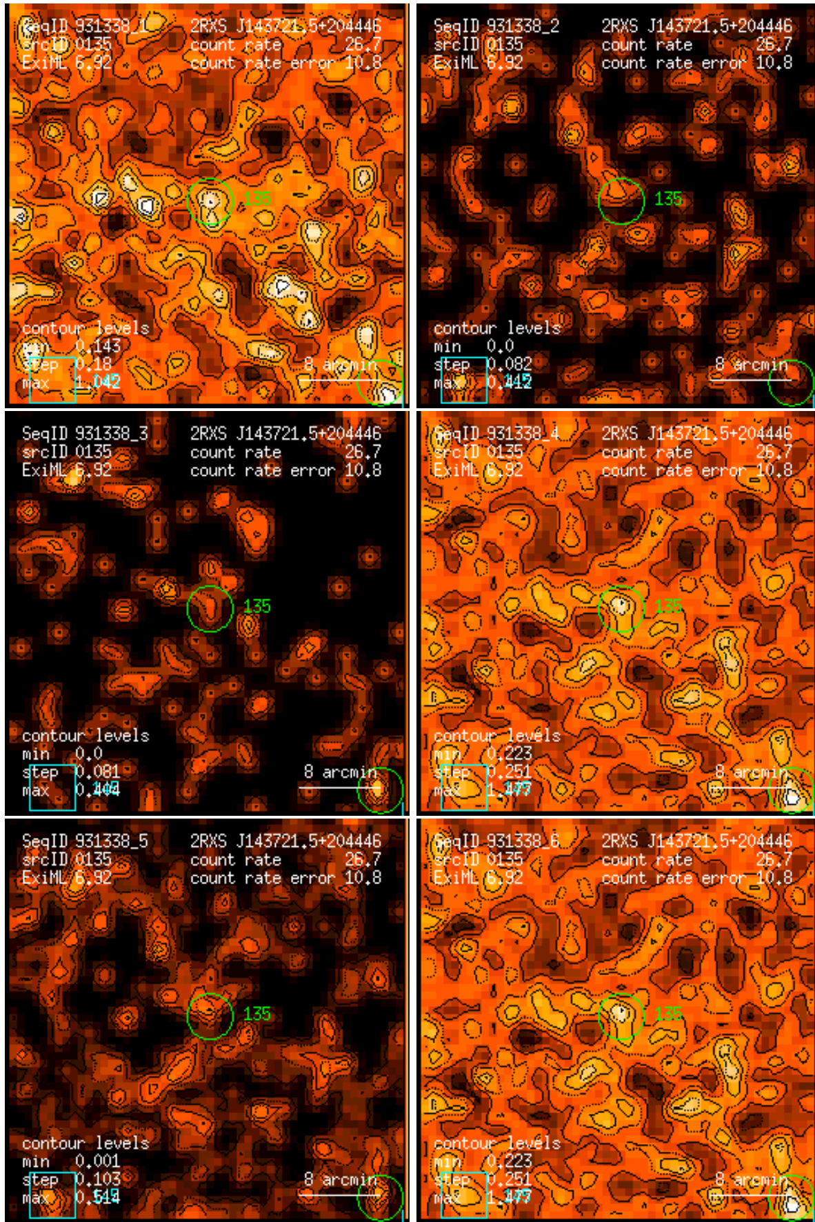
Figure 135: RASS 931338: detection 0135: band rate images, Gaussian filter: (1) PSPC channels 11 – 41, (2) 52 – 90, (3) 91 – 201, (4) 11 – 235, (5) 52 – 201, (6) 11 – 201. Broad band rates in counts/ks. Band rate contour levels in counts/ks/arcmin 2 .
