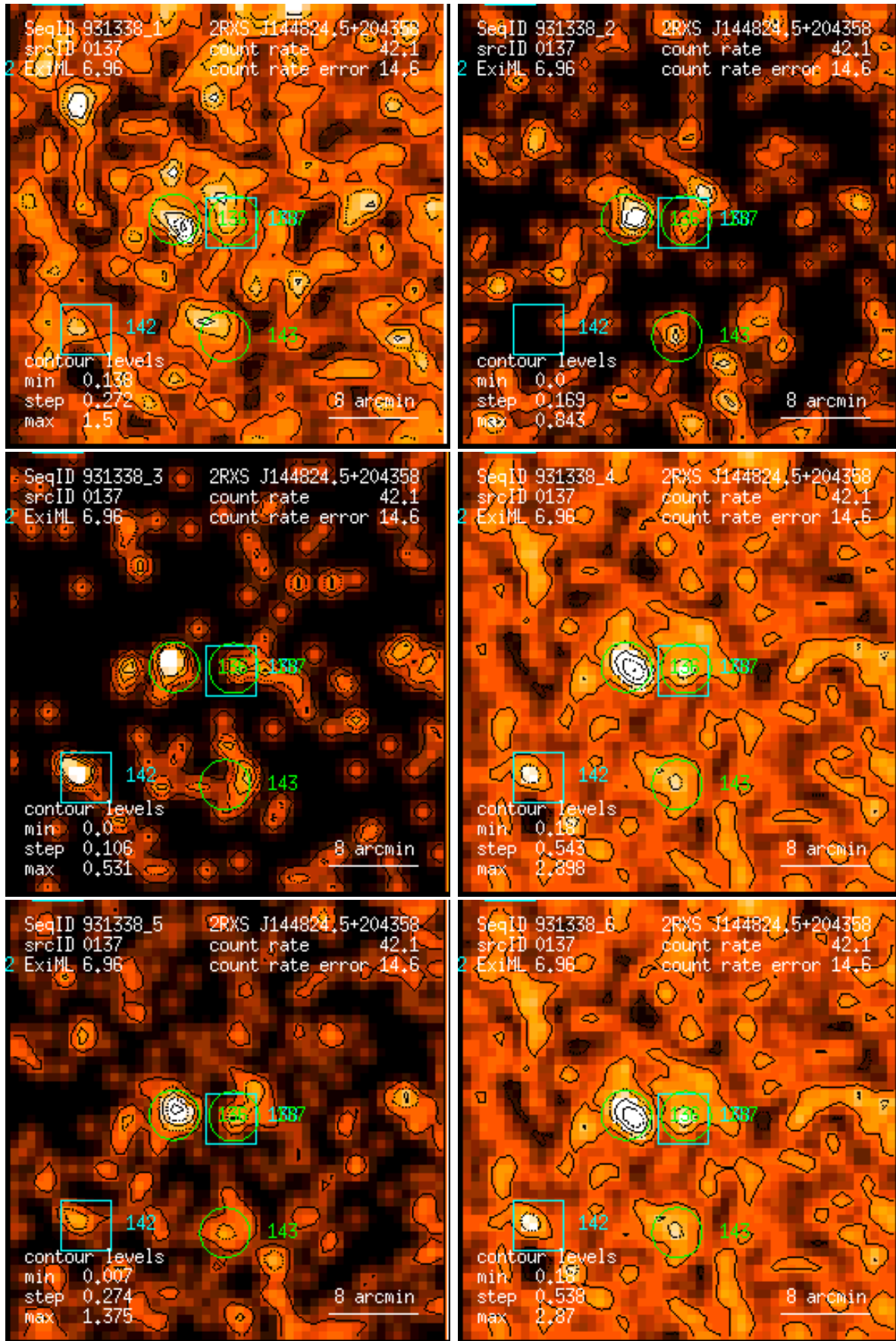
Figure 137: RASS 931338: detection 0137: band rate images, Gaussian filter: (1) PSPC channels 11 – 41, (2) 52 – 90, (3) 91 – 201, (4) 11 – 235, (5) 52 – 201, (6) 11 – 201. Broad band rates in counts/ks. Band rate contour levels in counts/ks/arcmin 2 .
