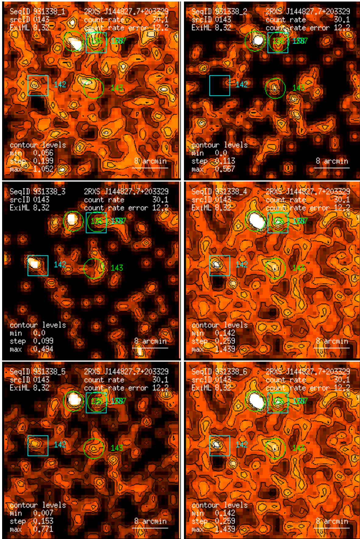
Figure 143: RASS 931338: detection 0143: band rate images, Gaussian filter: (1) PSPC channels 11 – 41, (2) 52 – 90, (3) 91 – 201, (4) 11 – 235, (5) 52 – 201, (6) 11 – 201. Broad band rates in counts/ks. Band rate contour levels in counts/ks/arcmin 2 .
