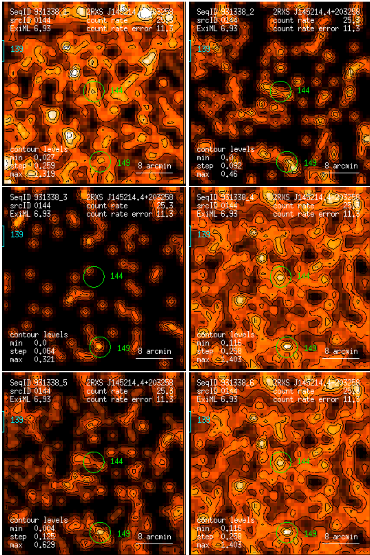
Figure 144: RASS 931338: detection 0144: band rate images, Gaussian filter: (1) PSPC channels 11 – 41, (2) 52 – 90, (3) 91 – 201, (4) 11 – 235, (5) 52 – 201, (6) 11 – 201. Broad band rates in counts/ks. Band rate contour levels in counts/ks/arcmin 2 .
