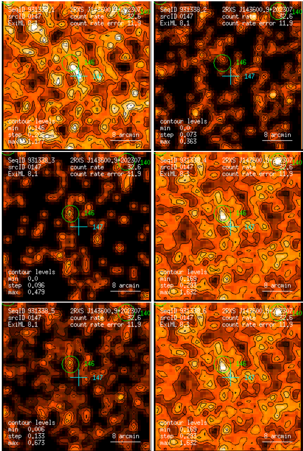
Figure 147: RASS 931338: detection 0147: band rate images, Gaussian filter: (1) PSPC channels 11 – 41, (2) 52 – 90, (3) 91 – 201, (4) 11 – 235, (5) 52 – 201, (6) 11 – 201. Broad band rates in counts/ks. Band rate contour levels in counts/ks/arcmin 2 .
