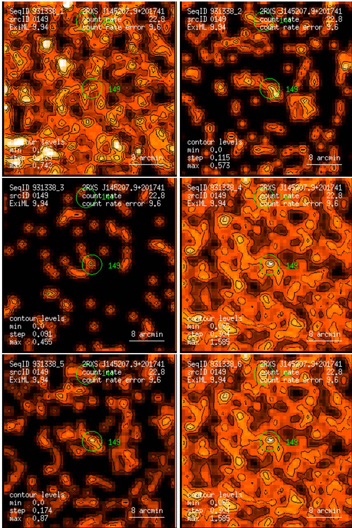
Figure 149: RASS 931338: detection 0149: band rate images, Gaussian filter: (1) PSPC channels 11 – 41, (2) 52 – 90, (3) 91 – 201, (4) 11 – 235, (5) 52 – 201, (6) 11 – 201. Broad band rates in counts/ks. Band rate contour levels in counts/ks/arcmin 2 .
