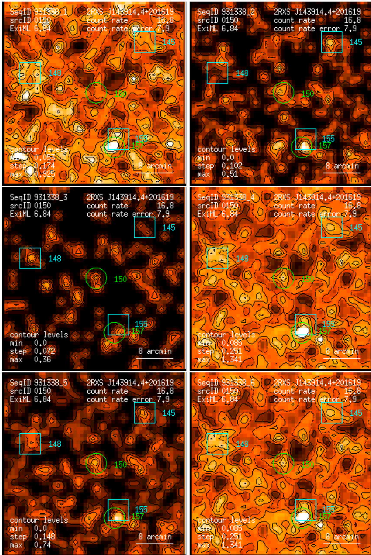
Figure 150: RASS 931338: detection 0150: band rate images, Gaussian filter: (1) PSPC channels 11 – 41, (2) 52 – 90, (3) 91 – 201, (4) 11 – 235, (5) 52 – 201, (6) 11 – 201. Broad band rates in counts/ks. Band rate contour levels in counts/ks/arcmin 2 .
