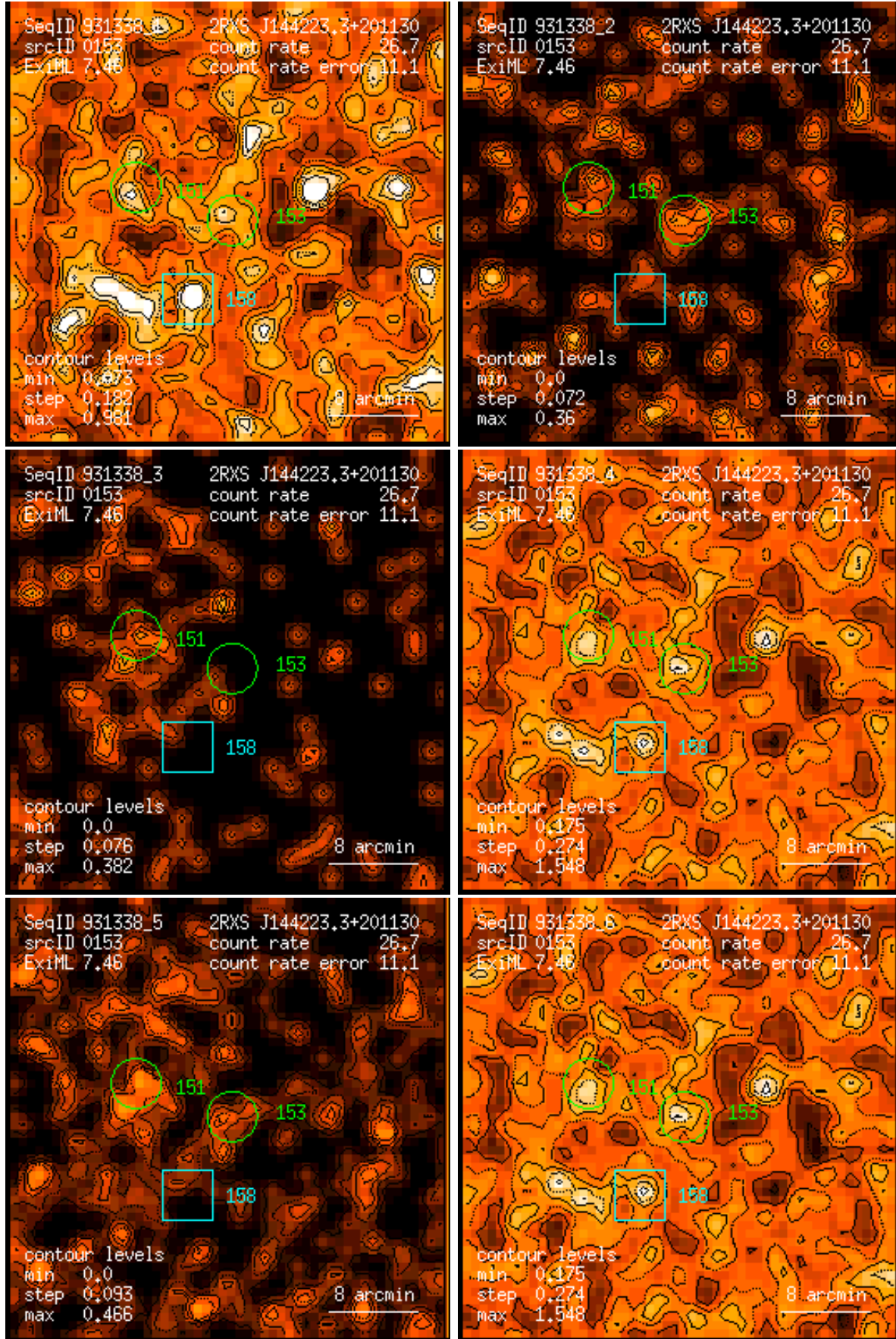
Figure 153: RASS 931338: detection 0153: band rate images, Gaussian filter: (1) PSPC channels 11 – 41, (2) 52 – 90, (3) 91 – 201, (4) 11 – 235, (5) 52 – 201, (6) 11 – 201. Broad band rates in counts/ks. Band rate contour levels in counts/ks/arcmin 2 .
