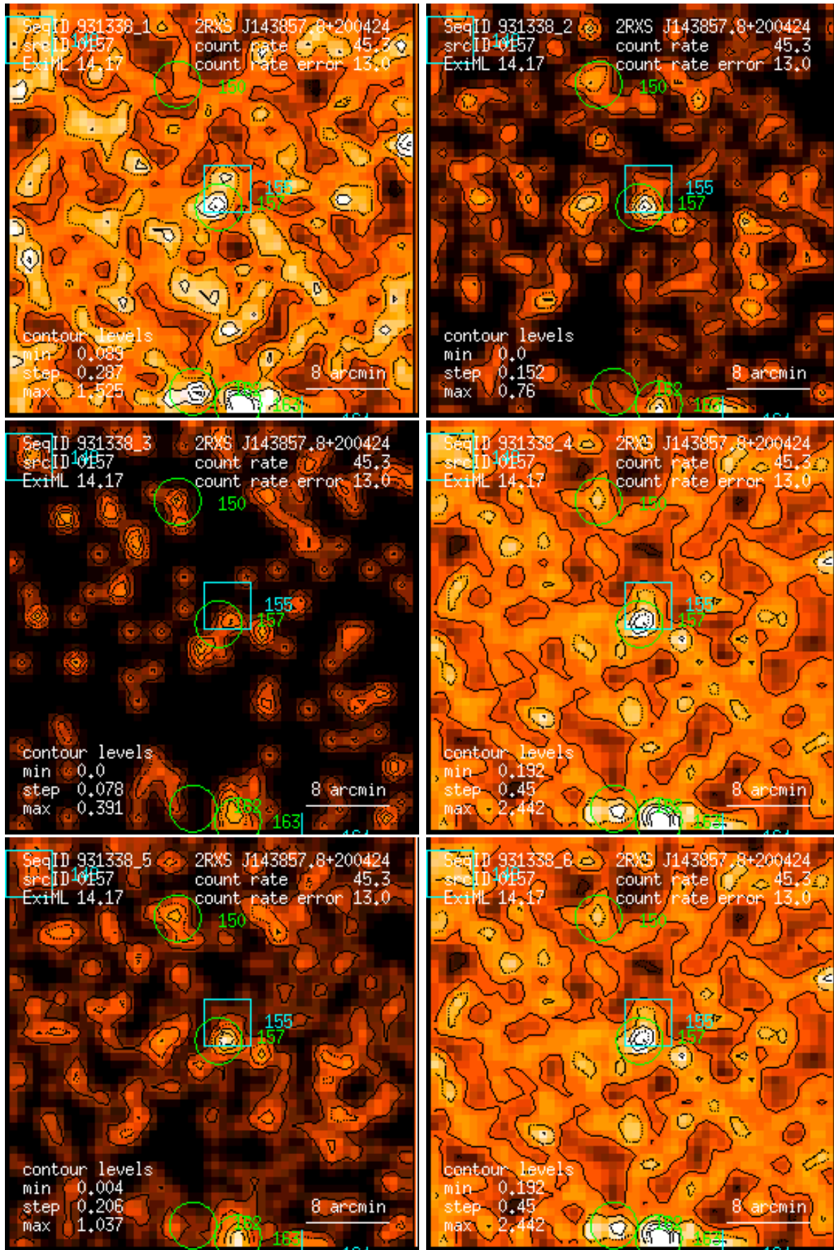
Figure 157: RASS 931338: detection 0157: band rate images, Gaussian filter: (1) PSPC channels 11 – 41, (2) 52 – 90, (3) 91 – 201, (4) 11 – 235, (5) 52 – 201, (6) 11 – 201. Broad band rates in counts/ks. Band rate contour levels in counts/ks/arcmin 2 .
