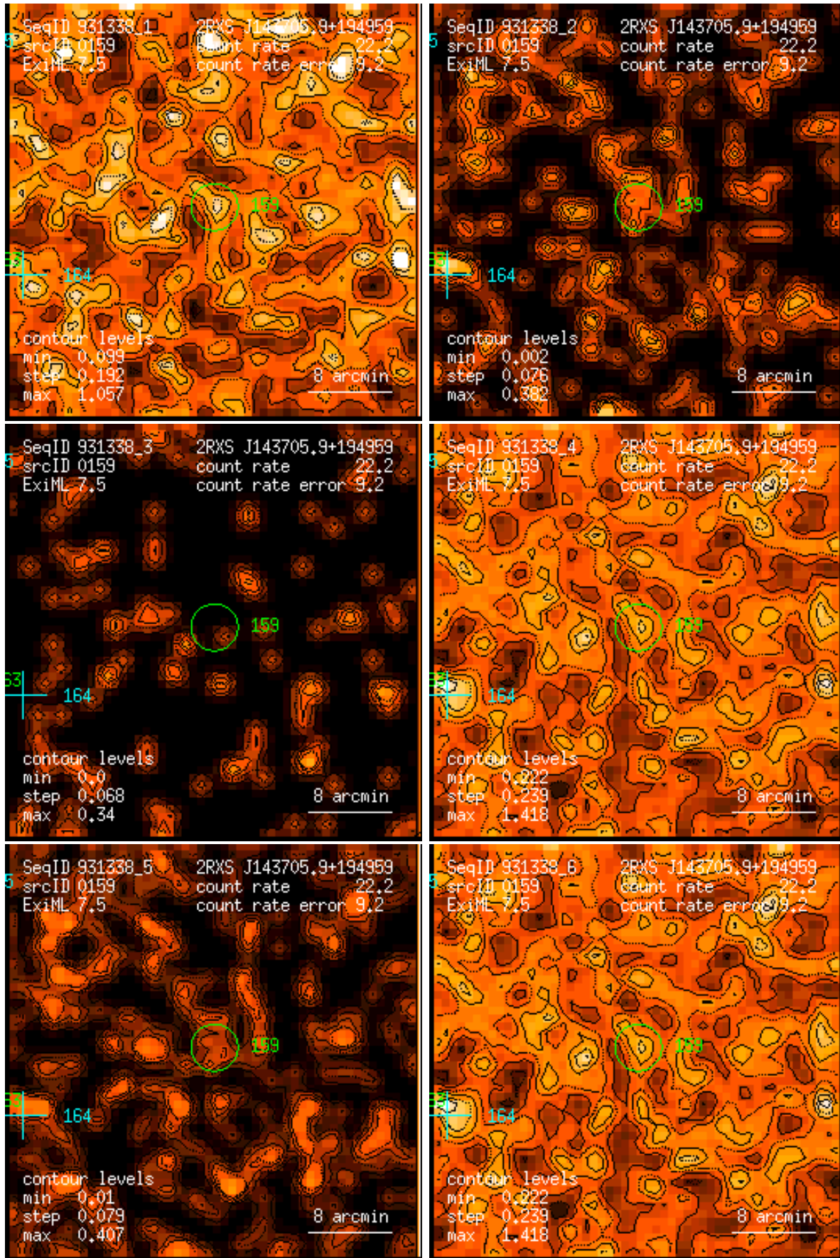
Figure 159: RASS 931338: detection 0159: band rate images, Gaussian filter: (1) PSPC channels 11 – 41, (2) 52 – 90, (3) 91 – 201, (4) 11 – 235, (5) 52 – 201, (6) 11 – 201. Broad band rates in counts/ks. Band rate contour levels in counts/ks/arcmin 2 .
