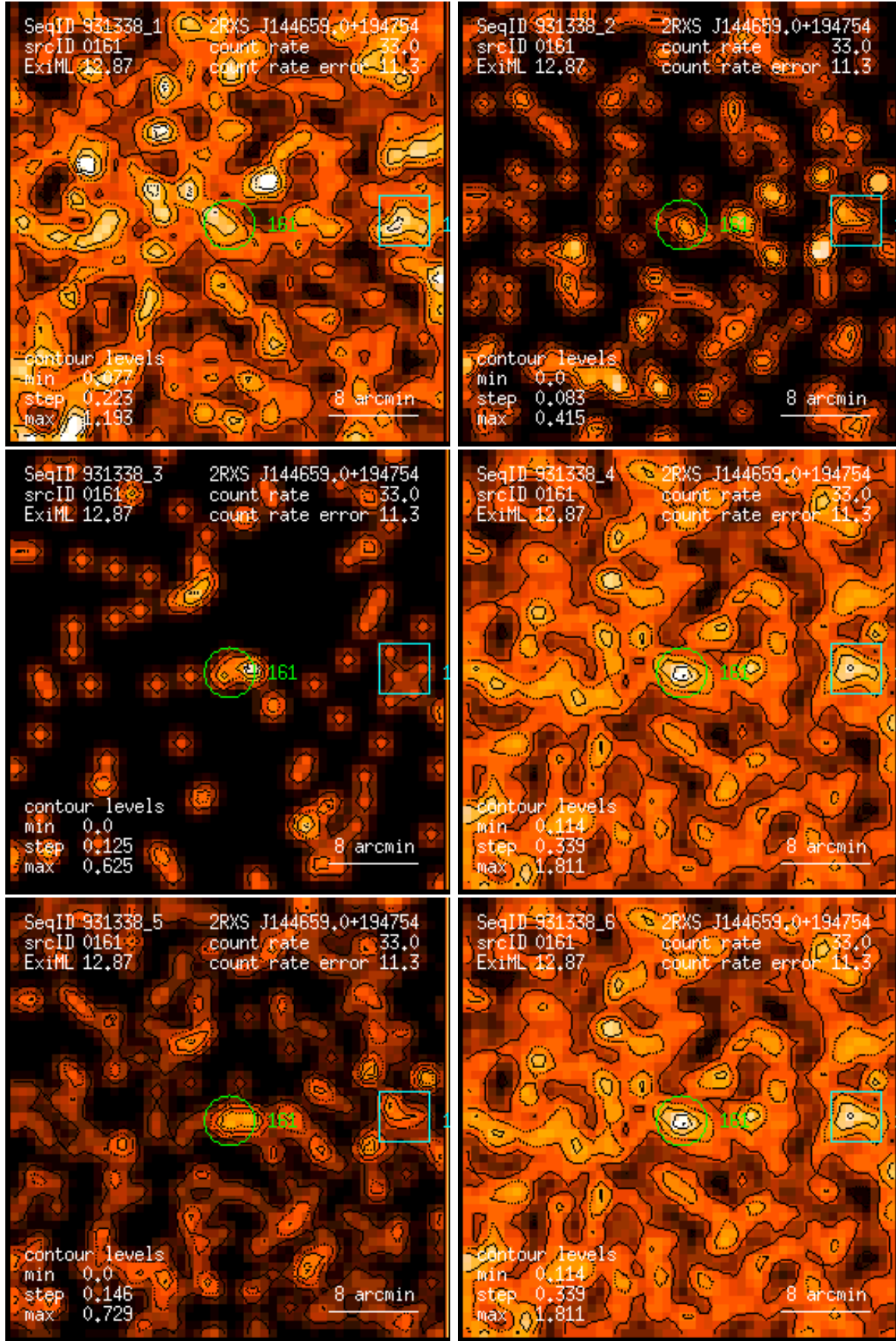
Figure 161: RASS 931338: detection 0161: band rate images, Gaussian filter: (1) PSPC channels 11 – 41, (2) 52 – 90, (3) 91 – 201, (4) 11 – 235, (5) 52 – 201, (6) 11 – 201. Broad band rates in counts/ks. Band rate contour levels in counts/ks/arcmin 2 .
