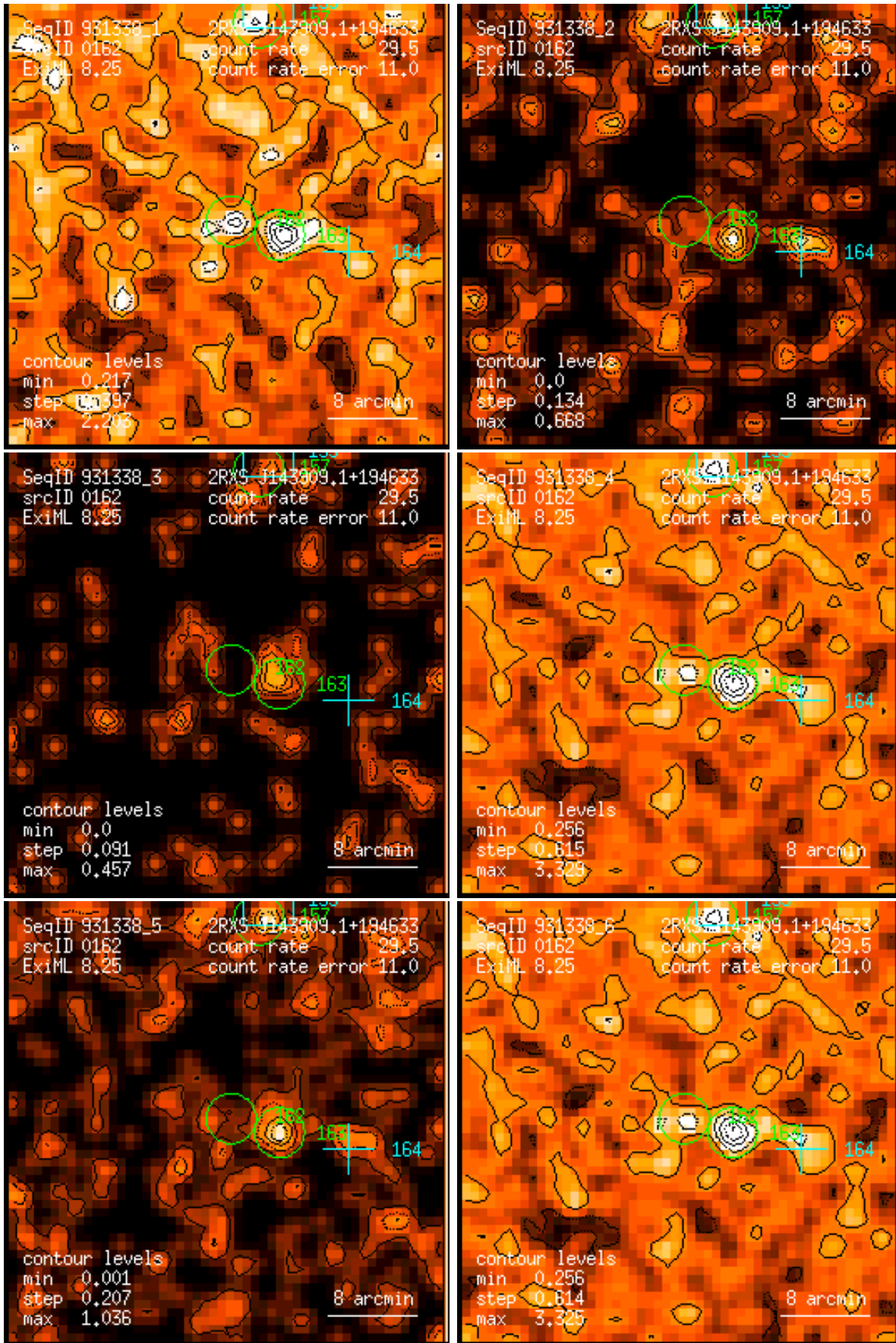
Figure 162: RASS 931338: detection 0162: band rate images, Gaussian filter: (1) PSPC channels 11 – 41, (2) 52 – 90, (3) 91 – 201, (4) 11 – 235, (5) 52 – 201, (6) 11 – 201. Broad band rates in counts/ks. Band rate contour levels in counts/ks/arcmin 2 .
