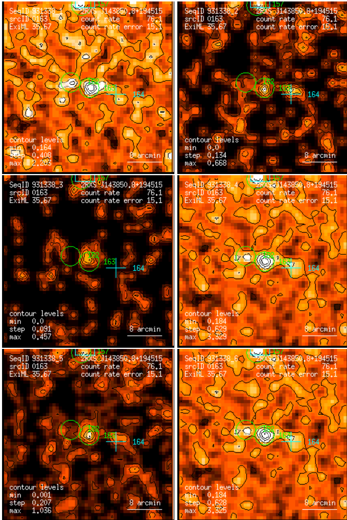
Figure 163: RASS 931338: detection 0163: band rate images, Gaussian filter: (1) PSPC channels 11 – 41, (2) 52 – 90, (3) 91 – 201, (4) 11 – 235, (5) 52 – 201, (6) 11 – 201. Broad band rates in counts/ks. Band rate contour levels in counts/ks/arcmin 2 .
