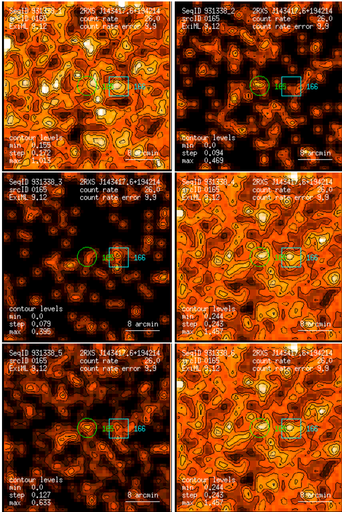
Figure 165: RASS 931338: detection 0165: band rate images, Gaussian filter: (1) PSPC channels 11 – 41, (2) 52 – 90, (3) 91 – 201, (4) 11 – 235, (5) 52 – 201, (6) 11 – 201. Broad band rates in counts/ks. Band rate contour levels in counts/ks/arcmin 2 .
