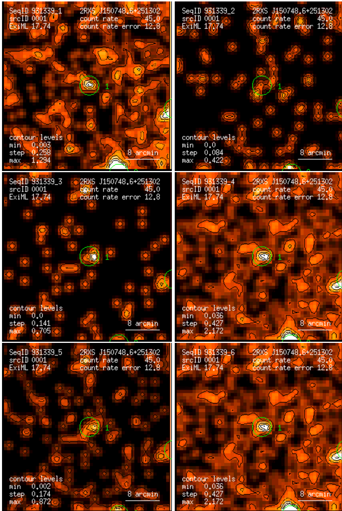
Figure 1: RASS 931339: detection 0001: band rate images, Gaussian filter: (1) PSPC channels 11 – 41, (2) 52 – 90, (3) 91 – 201, (4) 11 – 235, (5) 52 – 201, (6) 11 – 201. Broad band rates in counts/ks. Band rate contour levels in counts/ks/arcmin 2 .
