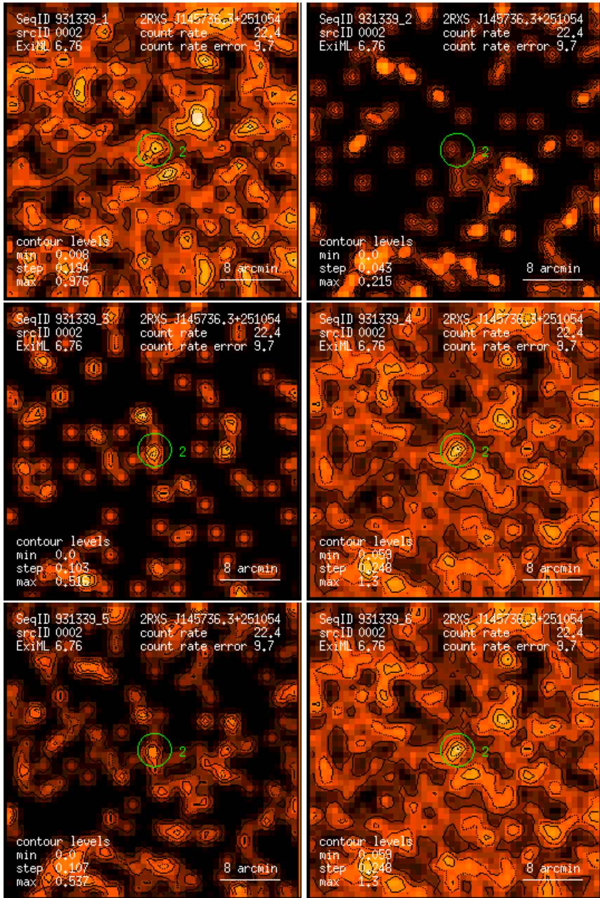
Figure 2: RASS 931339: detection 0002: band rate images, Gaussian filter: (1) PSPC channels 11 – 41, (2) 52 – 90, (3) 91 – 201, (4) 11 – 235, (5) 52 – 201, (6) 11 – 201. Broad band rates in counts/ks. Band rate contour levels in counts/ks/arcmin 2 .
