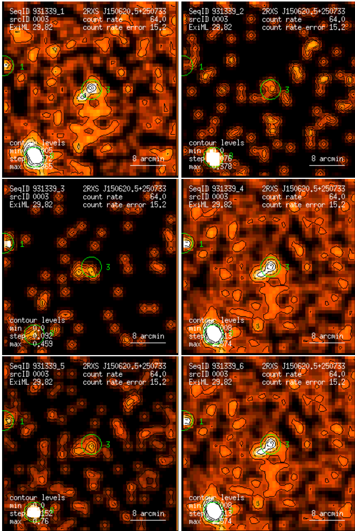
Figure 3: RASS 931339: detection 0003: band rate images, Gaussian filter: (1) PSPC channels 11 – 41, (2) 52 – 90, (3) 91 – 201, (4) 11 – 235, (5) 52 – 201, (6) 11 – 201. Broad band rates in counts/ks. Band rate contour levels in counts/ks/arcmin 2 .
