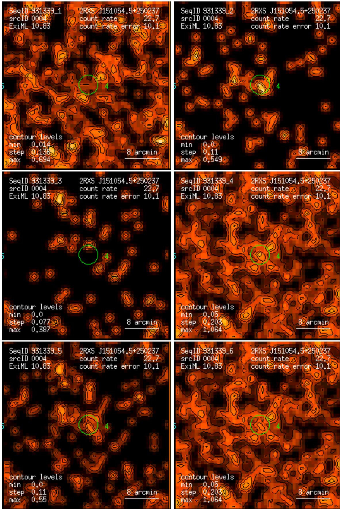
Figure 4: RASS 931339: detection 0004: band rate images, Gaussian filter: (1) PSPC channels 11 – 41, (2) 52 – 90, (3) 91 – 201, (4) 11 – 235, (5) 52 – 201, (6) 11 – 201. Broad band rates in counts/ks. Band rate contour levels in counts/ks/arcmin 2 .
