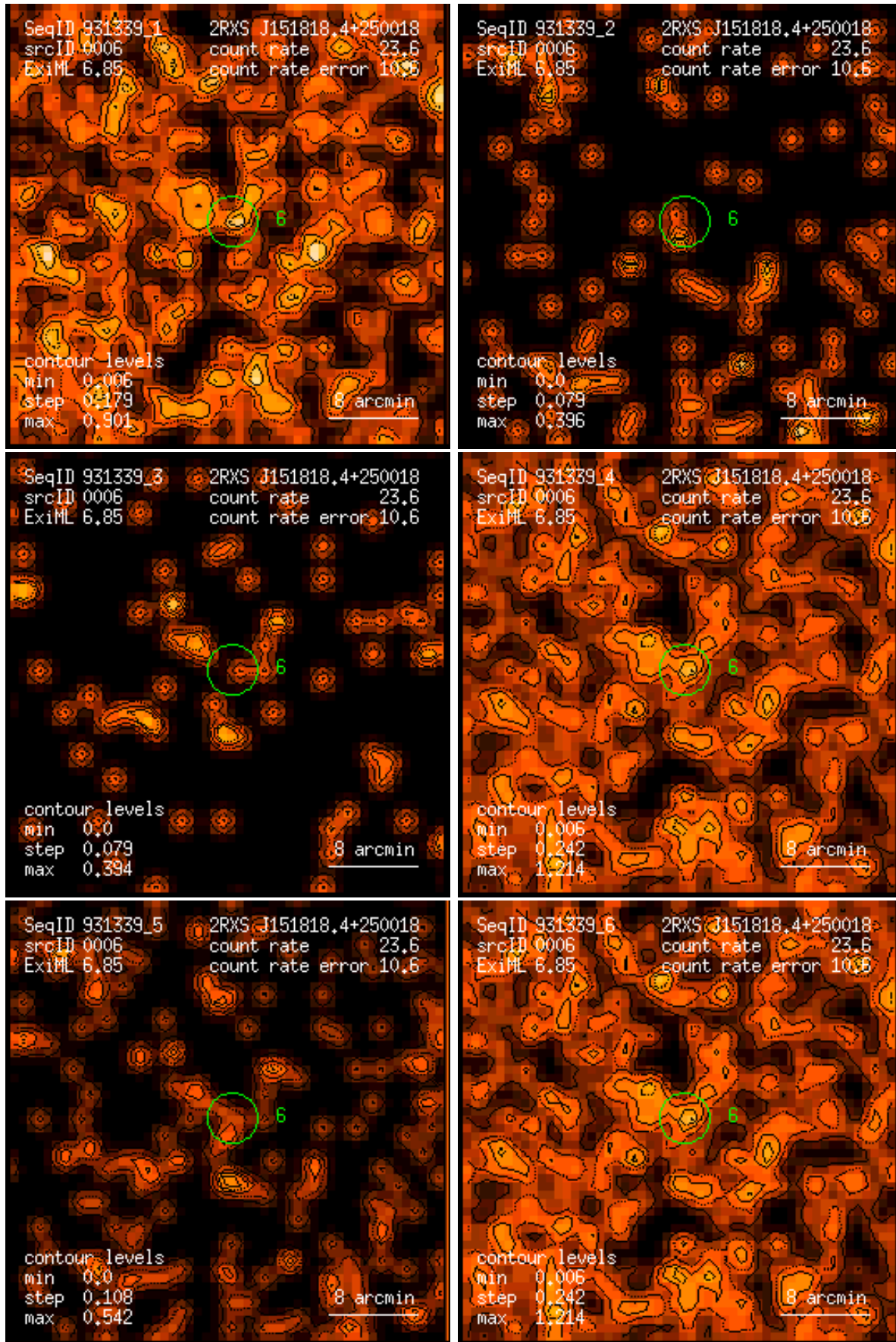
Figure 6: RASS 931339: detection 0006: band rate images, Gaussian filter: (1) PSPC channels 11 – 41, (2) 52 – 90, (3) 91 – 201, (4) 11 – 235, (5) 52 – 201, (6) 11 – 201. Broad band rates in counts/ks. Band rate contour levels in counts/ks/arcmin 2 .
