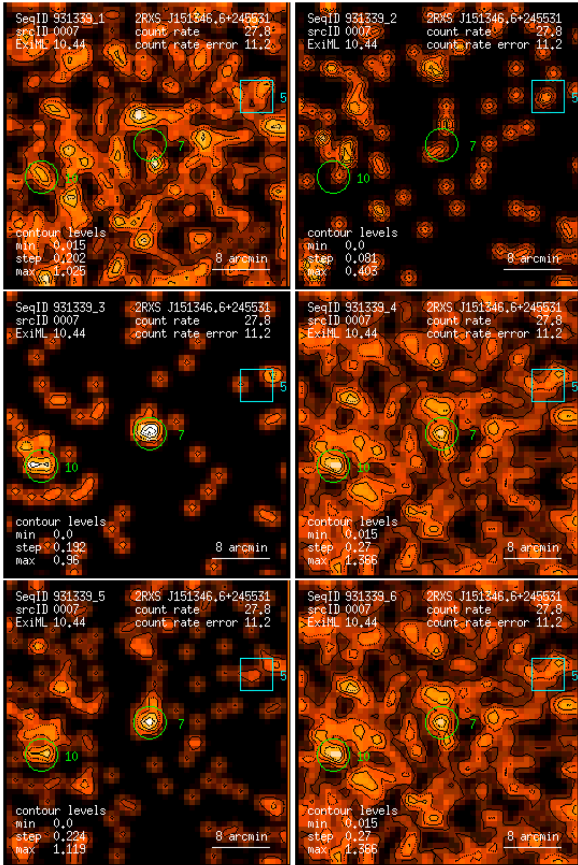
Figure 7: RASS 931339: detection 0007: band rate images, Gaussian filter: (1) PSPC channels 11 – 41, (2) 52 – 90, (3) 91 – 201, (4) 11 – 235, (5) 52 – 201, (6) 11 – 201. Broad band rates in counts/ks. Band rate contour levels in counts/ks/arcmin 2 .
