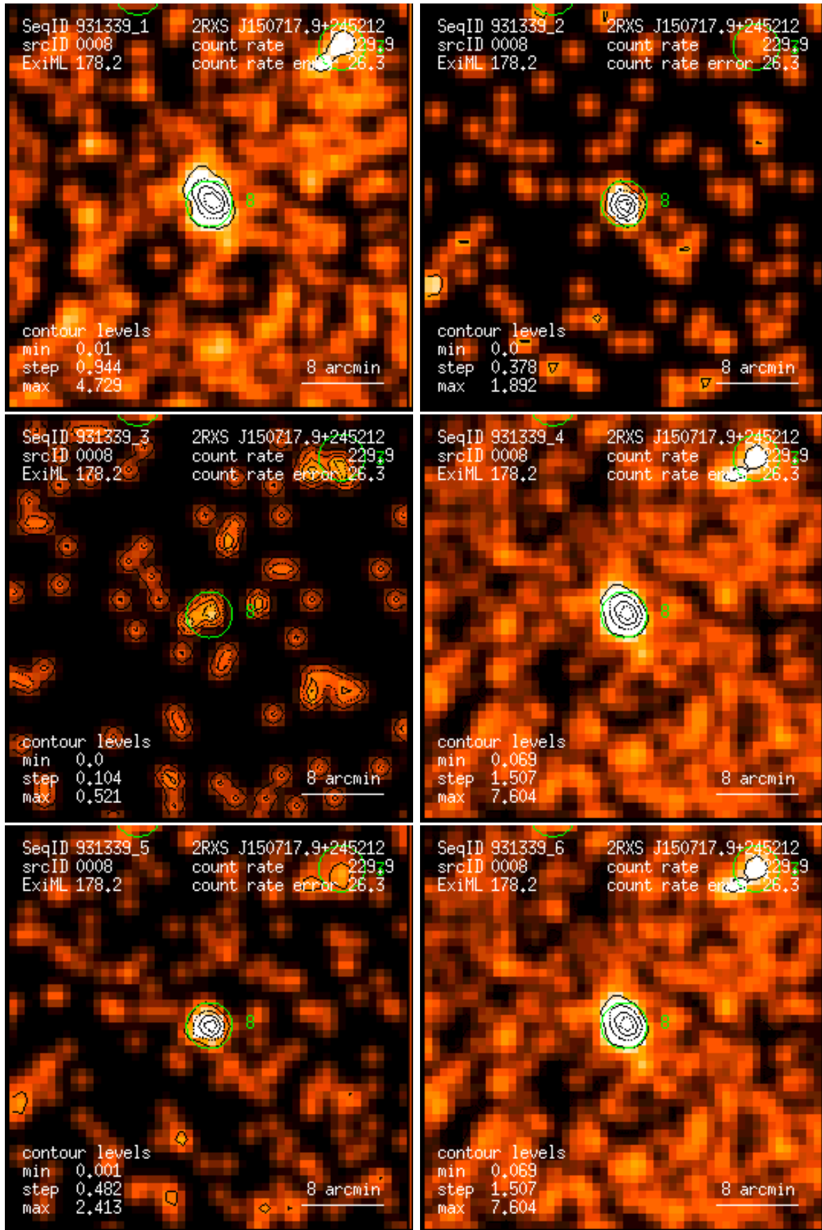
Figure 8: RASS 931339: detection 0008: band rate images, Gaussian filter: (1) PSPC channels 11 – 41, (2) 52 – 90, (3) 91 – 201, (4) 11 – 235, (5) 52 – 201, (6) 11 – 201. Broad band rates in counts/ks. Band rate contour levels in counts/ks/arcmin 2 .
