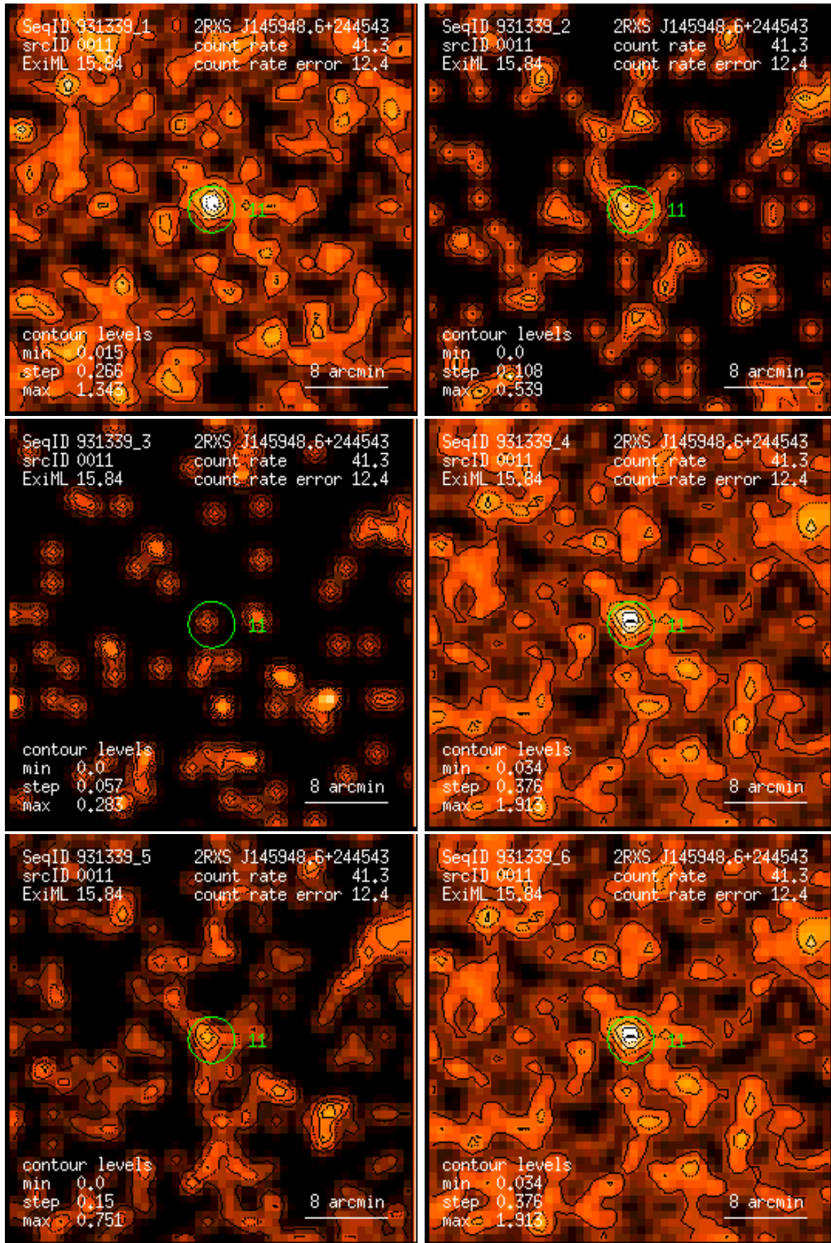
Figure 11: RASS 931339: detection 0011: band rate images, Gaussian filter: (1) PSPC channels 11 – 41, (2) 52 – 90, (3) 91 – 201, (4) 11 – 235, (5) 52 – 201, (6) 11 – 201. Broad band rates in counts/ks. Band rate contour levels in counts/ks/arcmin 2 .
