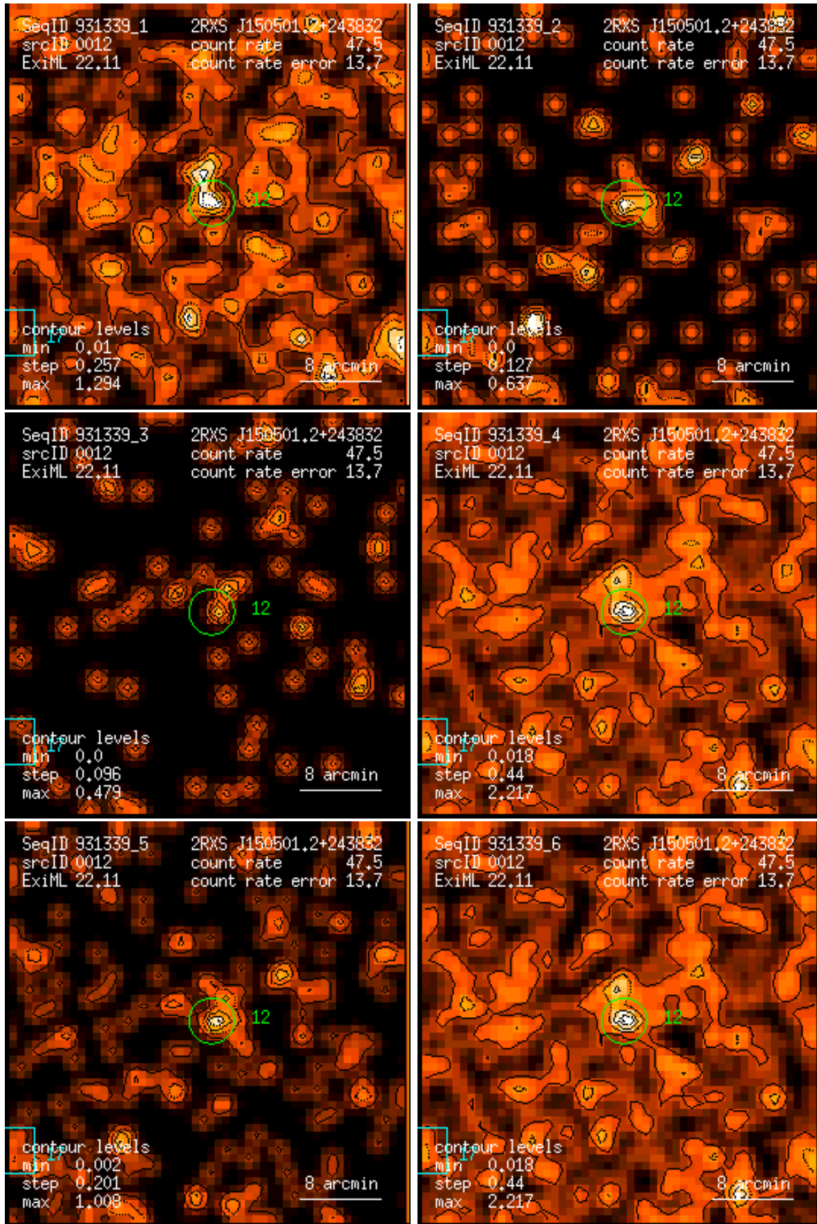
Figure 12: RASS 931339: detection 0012: band rate images, Gaussian filter: (1) PSPC channels 11 – 41, (2) 52 – 90, (3) 91 – 201, (4) 11 – 235, (5) 52 – 201, (6) 11 – 201. Broad band rates in counts/ks. Band rate contour levels in counts/ks/arcmin 2 .
