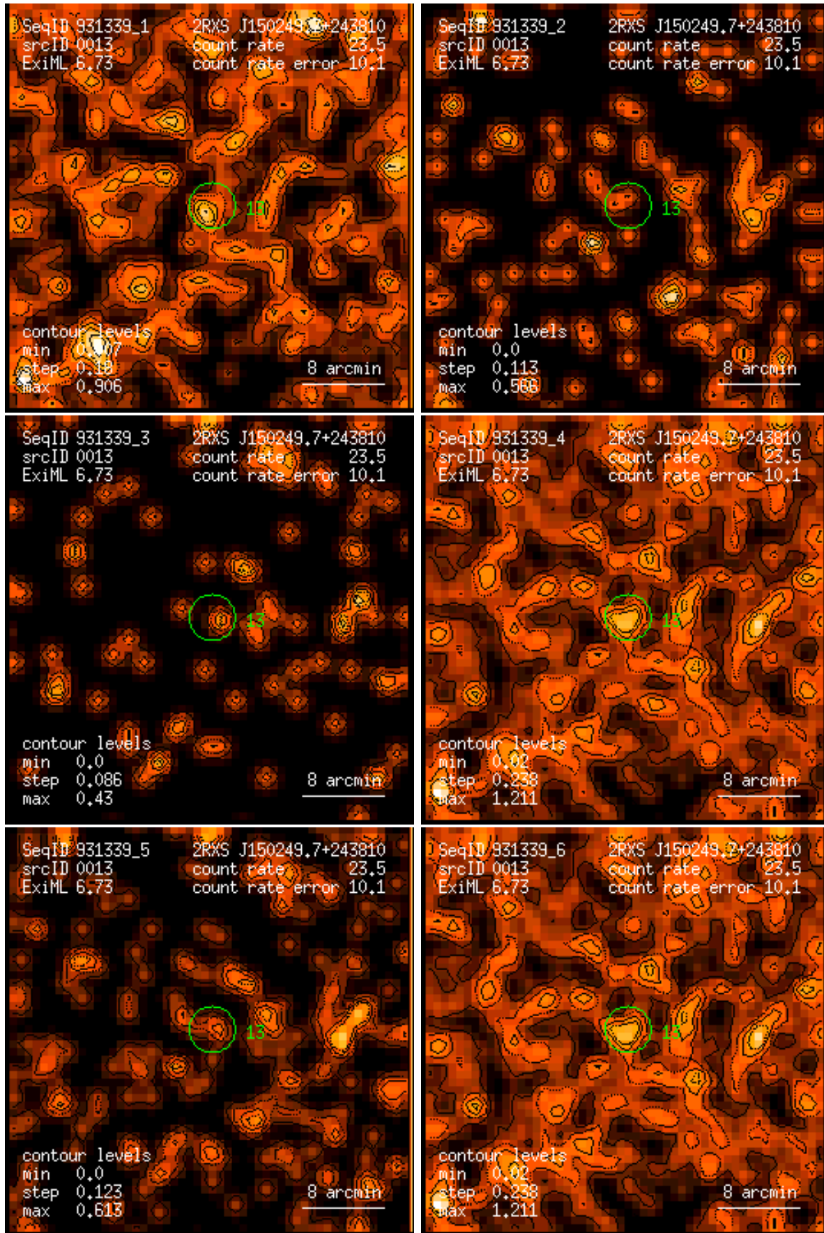
Figure 13: RASS 931339: detection 0013: band rate images, Gaussian filter: (1) PSPC channels 11 – 41, (2) 52 – 90, (3) 91 – 201, (4) 11 – 235, (5) 52 – 201, (6) 11 – 201. Broad band rates in counts/ks. Band rate contour levels in counts/ks/arcmin 2 .
