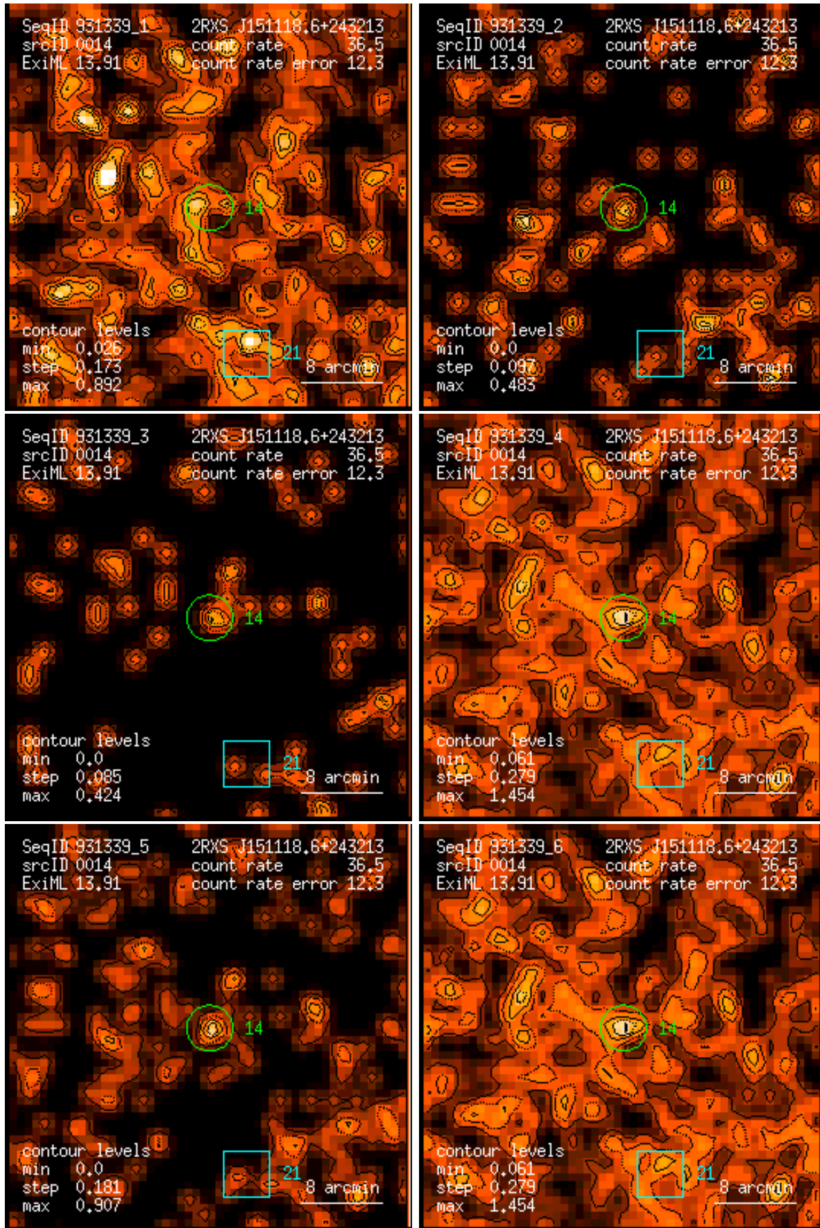
Figure 14: RASS 931339: detection 0014: band rate images, Gaussian filter: (1) PSPC channels 11 – 41, (2) 52 – 90, (3) 91 – 201, (4) 11 – 235, (5) 52 – 201, (6) 11 – 201. Broad band rates in counts/ks. Band rate contour levels in counts/ks/arcmin 2 .
