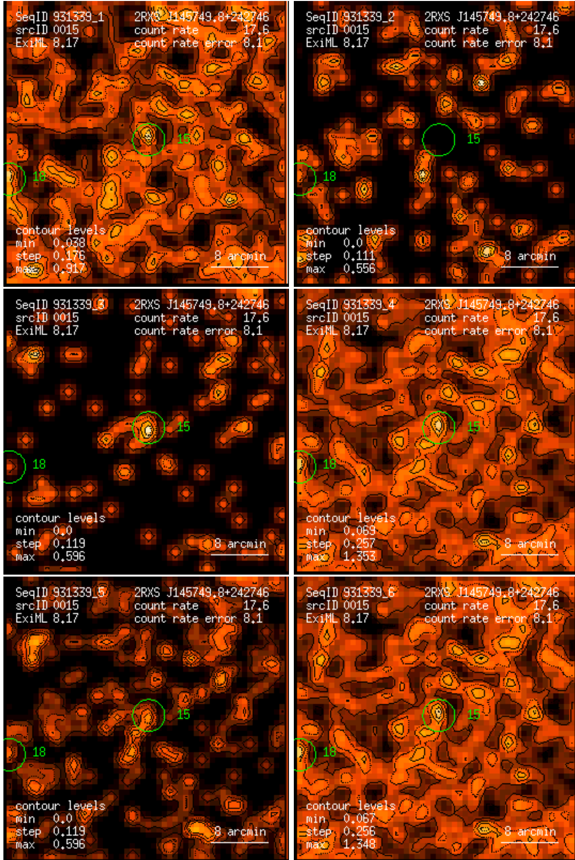
Figure 15: RASS 931339: detection 0015: band rate images, Gaussian filter: (1) PSPC channels 11 – 41, (2) 52 – 90, (3) 91 – 201, (4) 11 – 235, (5) 52 – 201, (6) 11 – 201. Broad band rates in counts/ks. Band rate contour levels in counts/ks/arcmin 2 .
