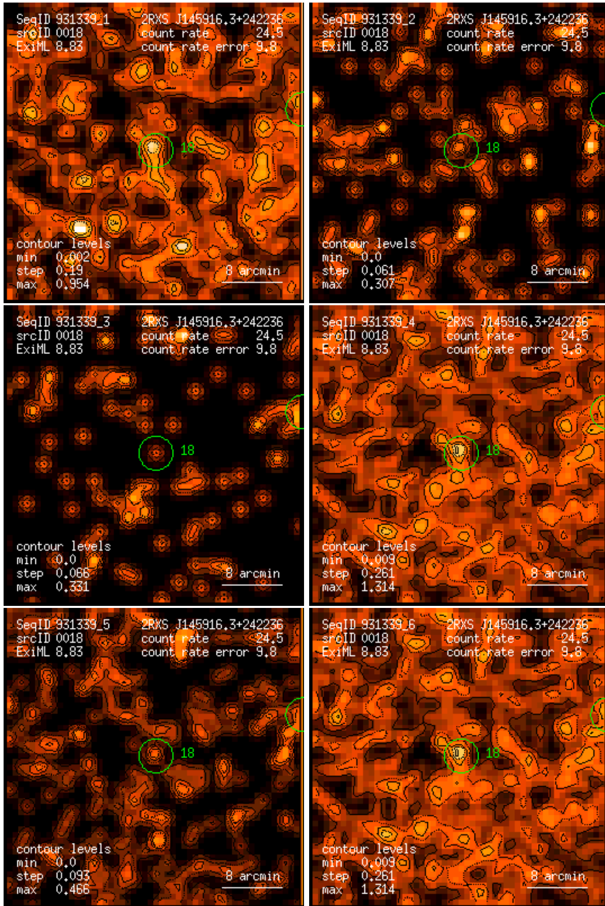
Figure 18: RASS 931339: detection 0018: band rate images, Gaussian filter: (1) PSPC channels 11 – 41, (2) 52 – 90, (3) 91 – 201, (4) 11 – 235, (5) 52 – 201, (6) 11 – 201. Broad band rates in counts/ks. Band rate contour levels in counts/ks/arcmin 2 .
