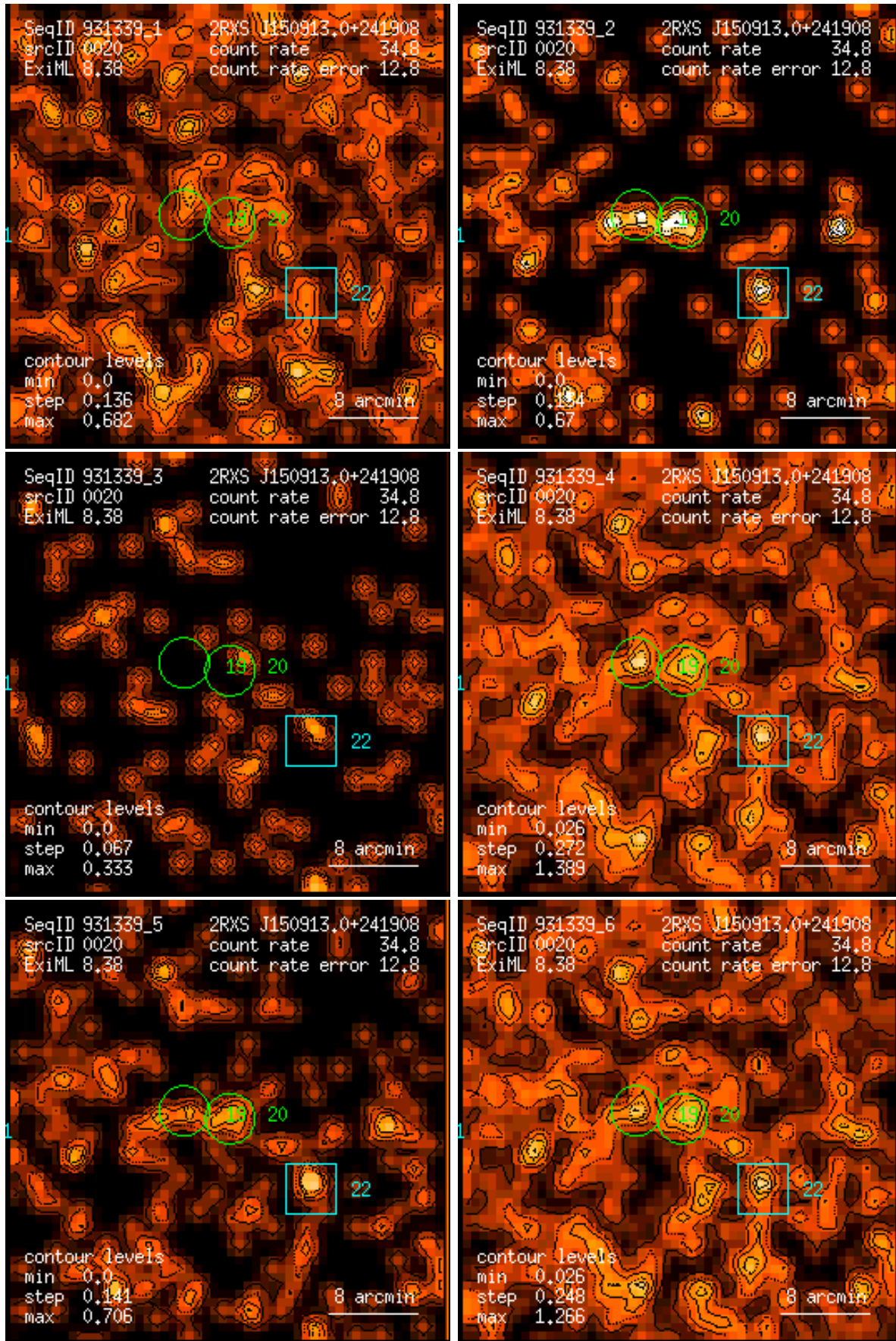
Figure 20: RASS 931339: detection 0020: band rate images, Gaussian filter: (1) PSPC channels 11 – 41, (2) 52 – 90, (3) 91 – 201, (4) 11 – 235, (5) 52 – 201, (6) 11 – 201. Broad band rates in counts/ks. Band rate contour levels in counts/ks/arcmin 2 .
