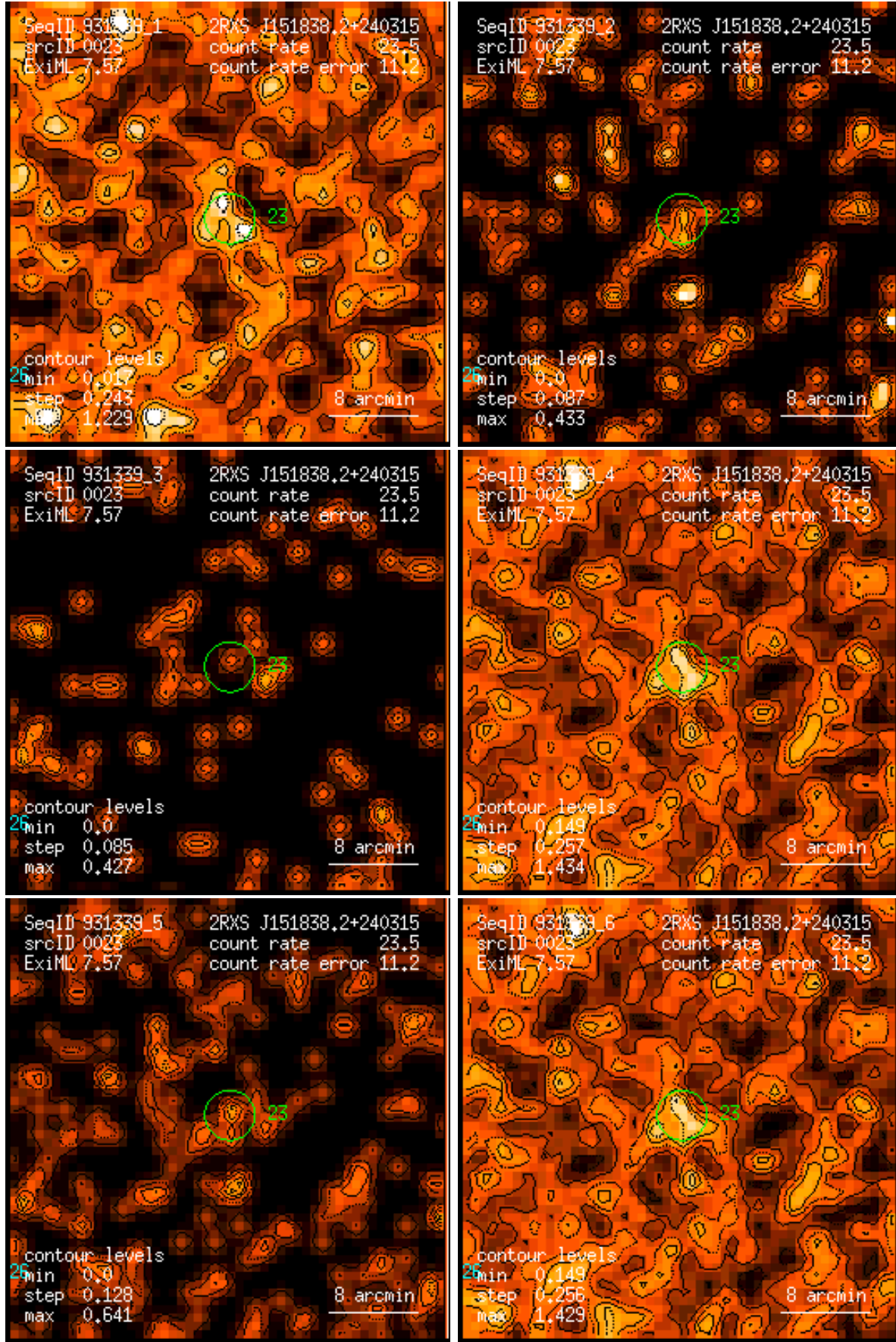
Figure 23: RASS 931339: detection 0023: band rate images, Gaussian filter: (1) PSPC channels 11 – 41, (2) 52 – 90, (3) 91 – 201, (4) 11 – 235, (5) 52 – 201, (6) 11 – 201. Broad band rates in counts/ks. Band rate contour levels in counts/ks/arcmin 2 .
