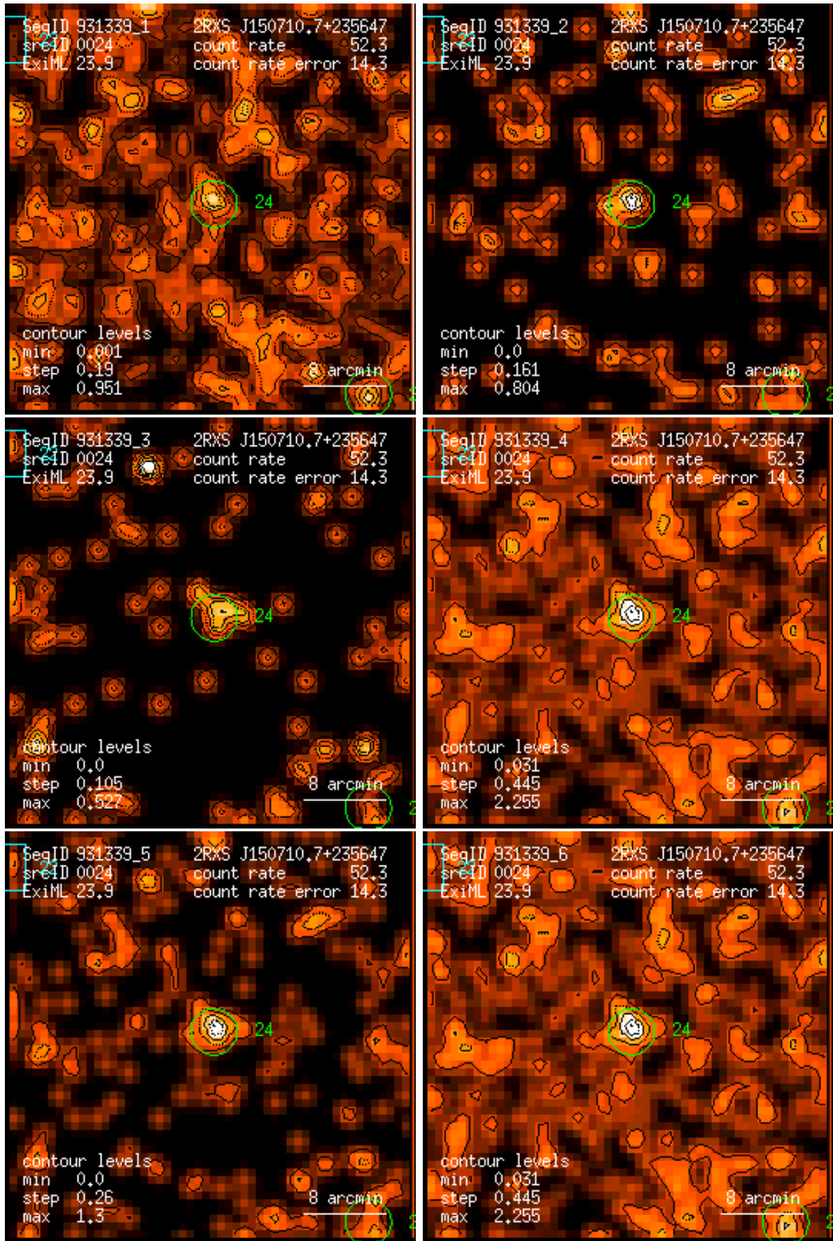
Figure 24: RASS 931339: detection 0024: band rate images, Gaussian filter: (1) PSPC channels 11 – 41, (2) 52 – 90, (3) 91 – 201, (4) 11 – 235, (5) 52 – 201, (6) 11 – 201. Broad band rates in counts/ks. Band rate contour levels in counts/ks/arcmin 2 .
