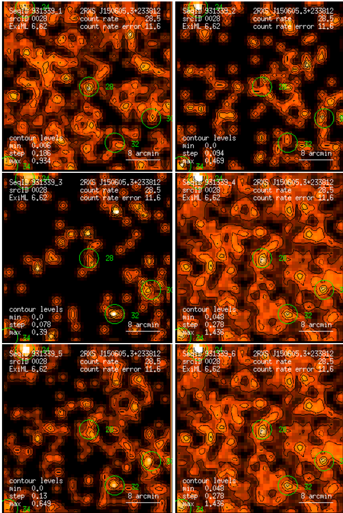
Figure 28: RASS 931339: detection 0028: band rate images, Gaussian filter: (1) PSPC channels 11 – 41, (2) 52 – 90, (3) 91 – 201, (4) 11 – 235, (5) 52 – 201, (6) 11 – 201. Broad band rates in counts/ks. Band rate contour levels in counts/ks/arcmin 2 .
