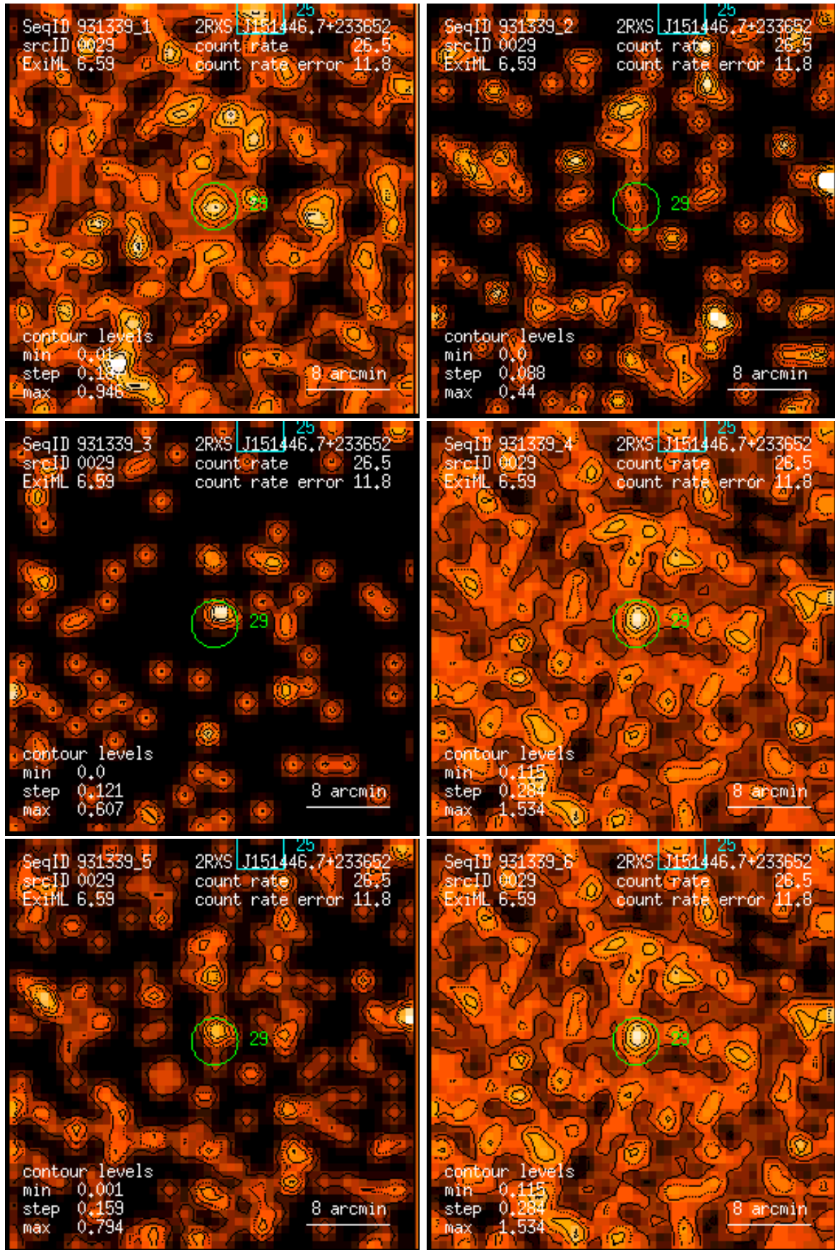
Figure 29: RASS 931339: detection 0029: band rate images, Gaussian filter: (1) PSPC channels 11 – 41, (2) 52 – 90, (3) 91 – 201, (4) 11 – 235, (5) 52 – 201, (6) 11 – 201. Broad band rates in counts/ks. Band rate contour levels in counts/ks/arcmin 2 .
