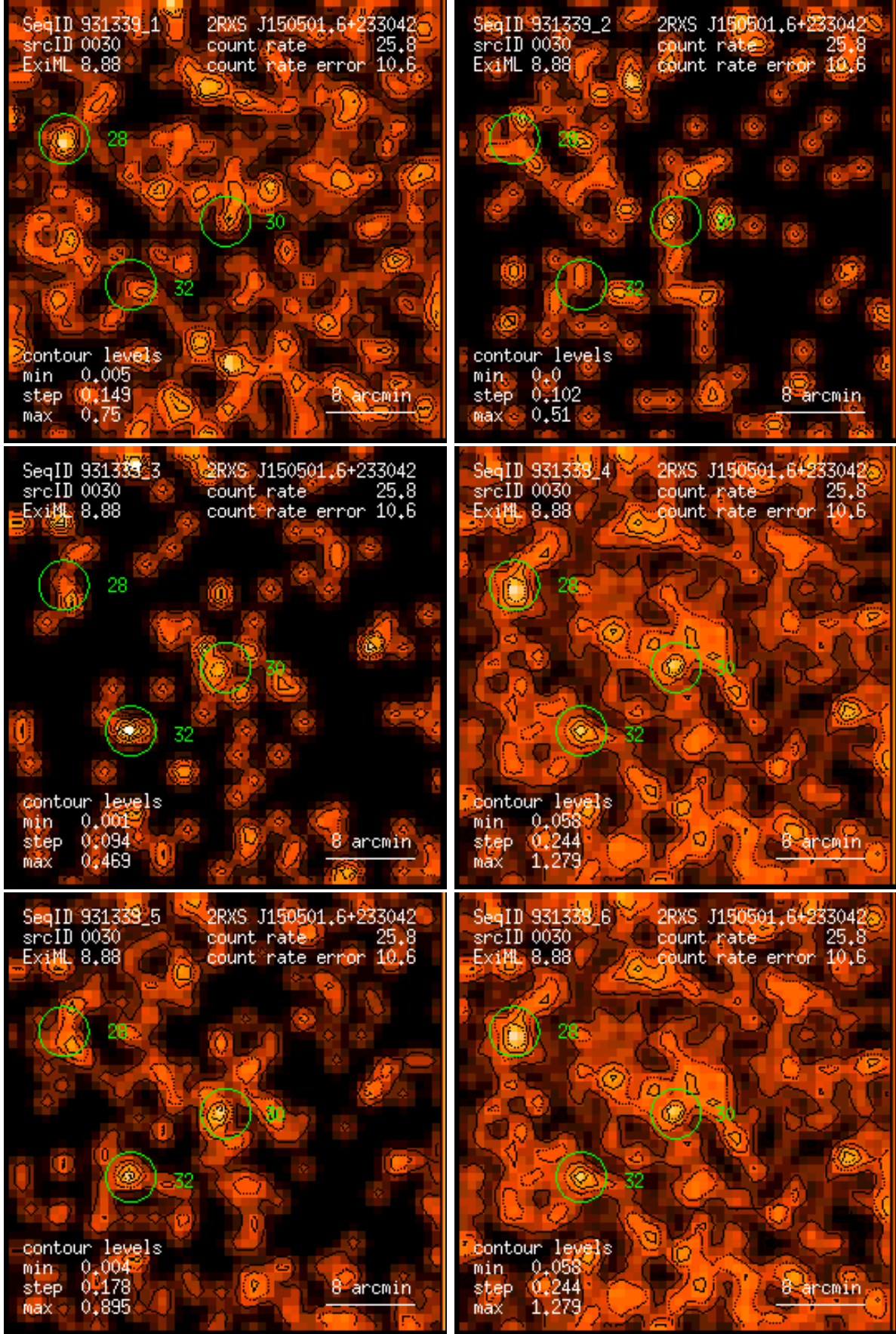
Figure 30: RASS 931339: detection 0030: band rate images, Gaussian filter: (1) PSPC channels 11 – 41, (2) 52 – 90, (3) 91 – 201, (4) 11 – 235, (5) 52 – 201, (6) 11 – 201. Broad band rates in counts/ks. Band rate contour levels in counts/ks/arcmin 2 .
