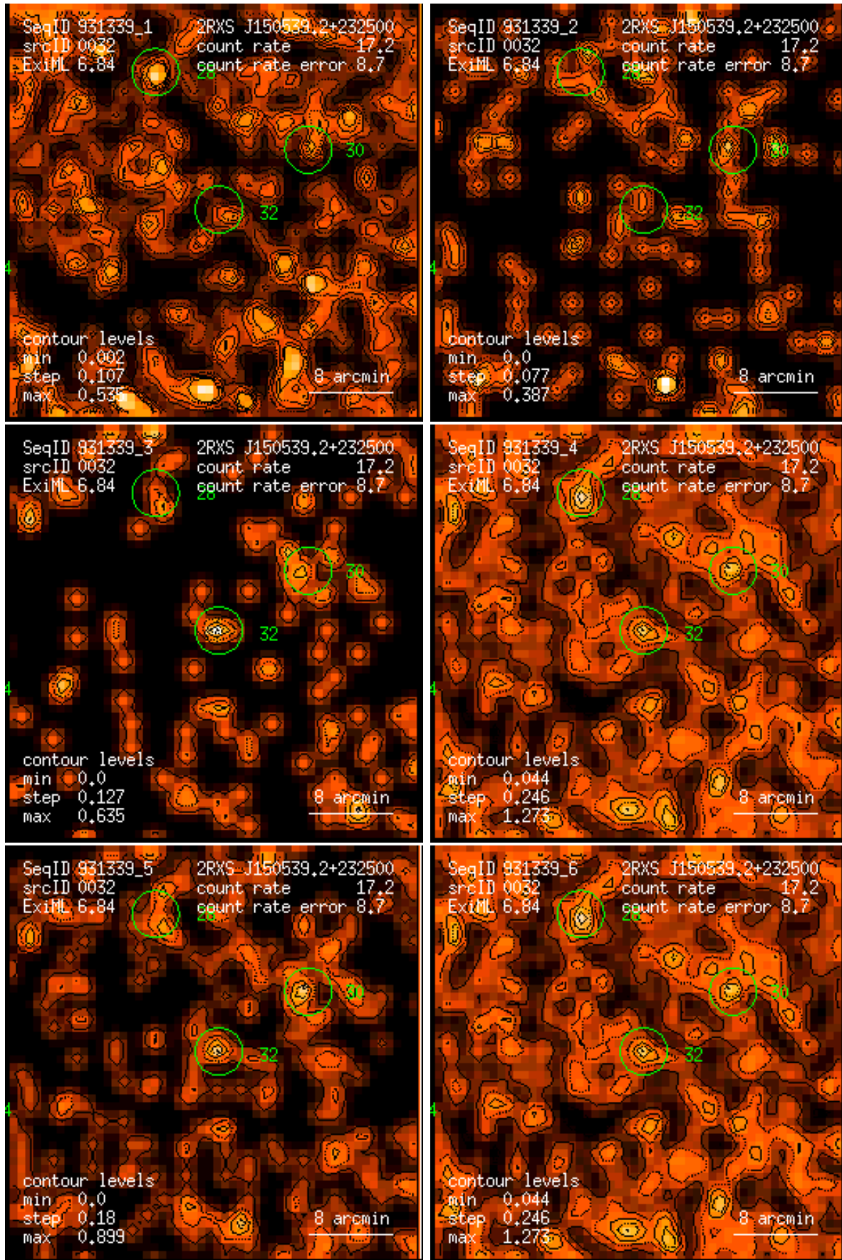
Figure 32: RASS 931339: detection 0032: band rate images, Gaussian filter: (1) PSPC channels 11 – 41, (2) 52 – 90, (3) 91 – 201, (4) 11 – 235, (5) 52 – 201, (6) 11 – 201. Broad band rates in counts/ks. Band rate contour levels in counts/ks/arcmin 2 .
